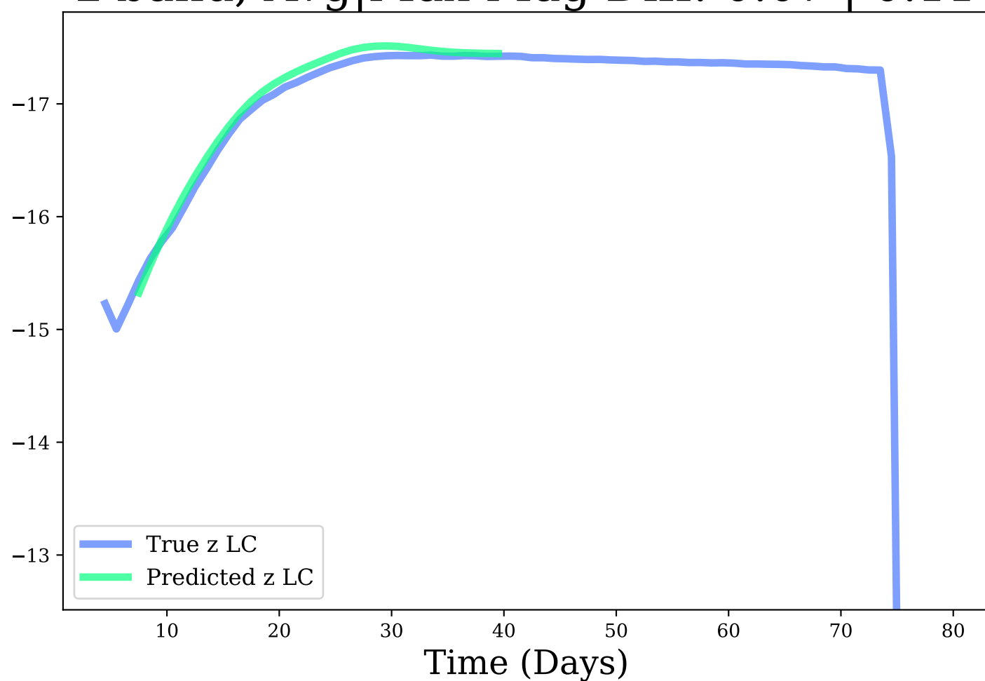
z-band, Avg|Max Mag Diff: 0.07 | 0.11
