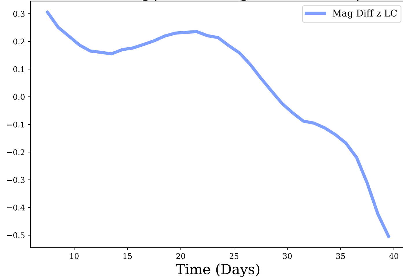
z-band, Avg|Max Mag Diff: 0.06 | 0.5
