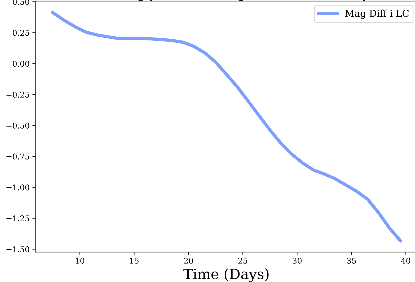
i-band, Avg|Max Mag Diff: -0.31 | 1.43
