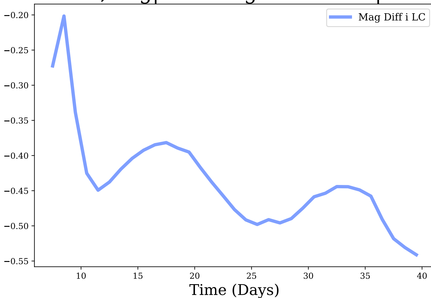
i-band, Avg|Max Mag Diff: -0.44 | 0.54
