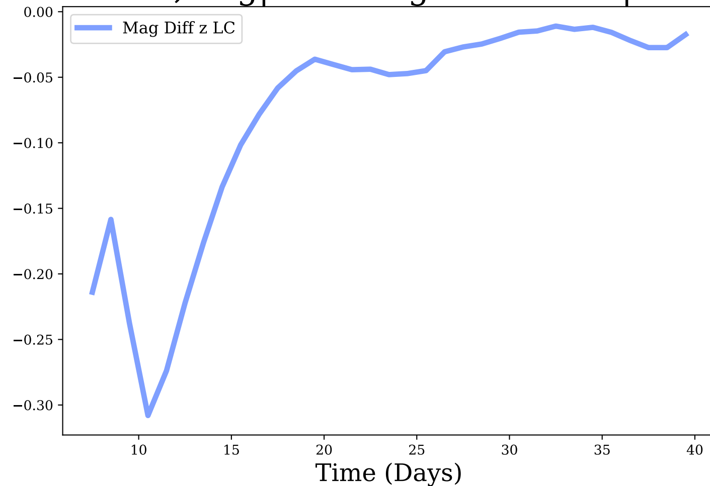
z-band, Avg|Max Mag Diff: -0.08 | 0.31
