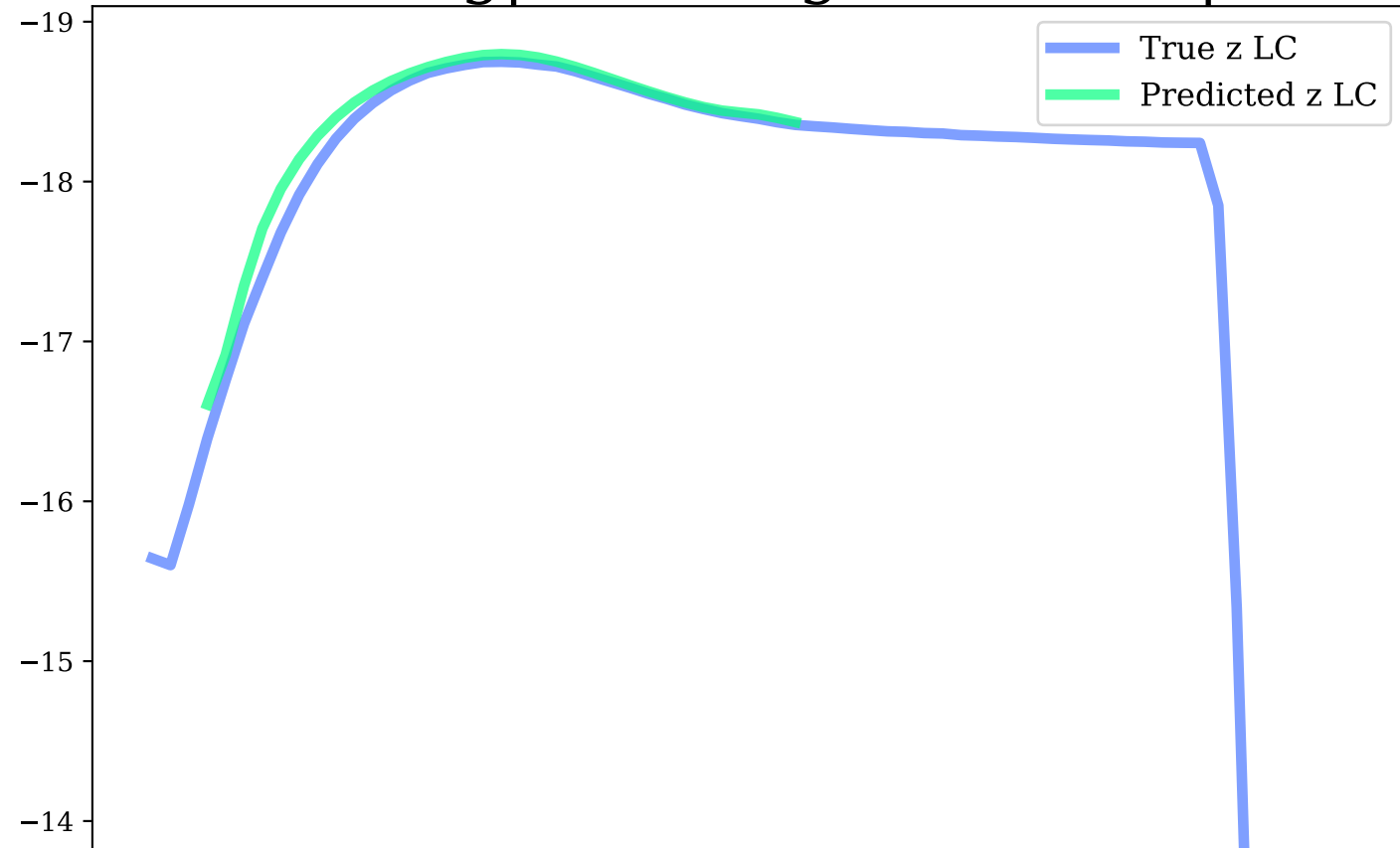
z-band, Avg|Max Mag Diff: 0.08 | 0.31
