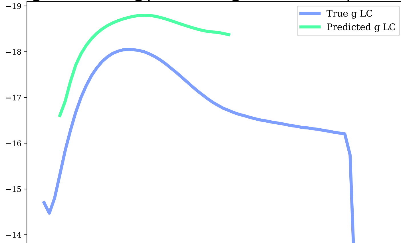
i-band, Avg|Max Mag Diff: 0.44 | 0.54
