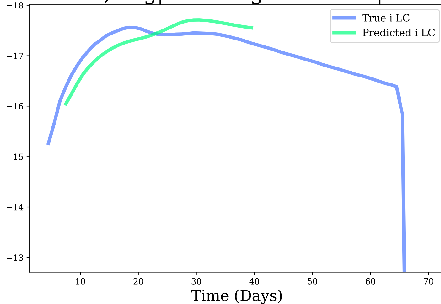
i-band, Avg|Max Mag Diff: 0.25 | 0.38
