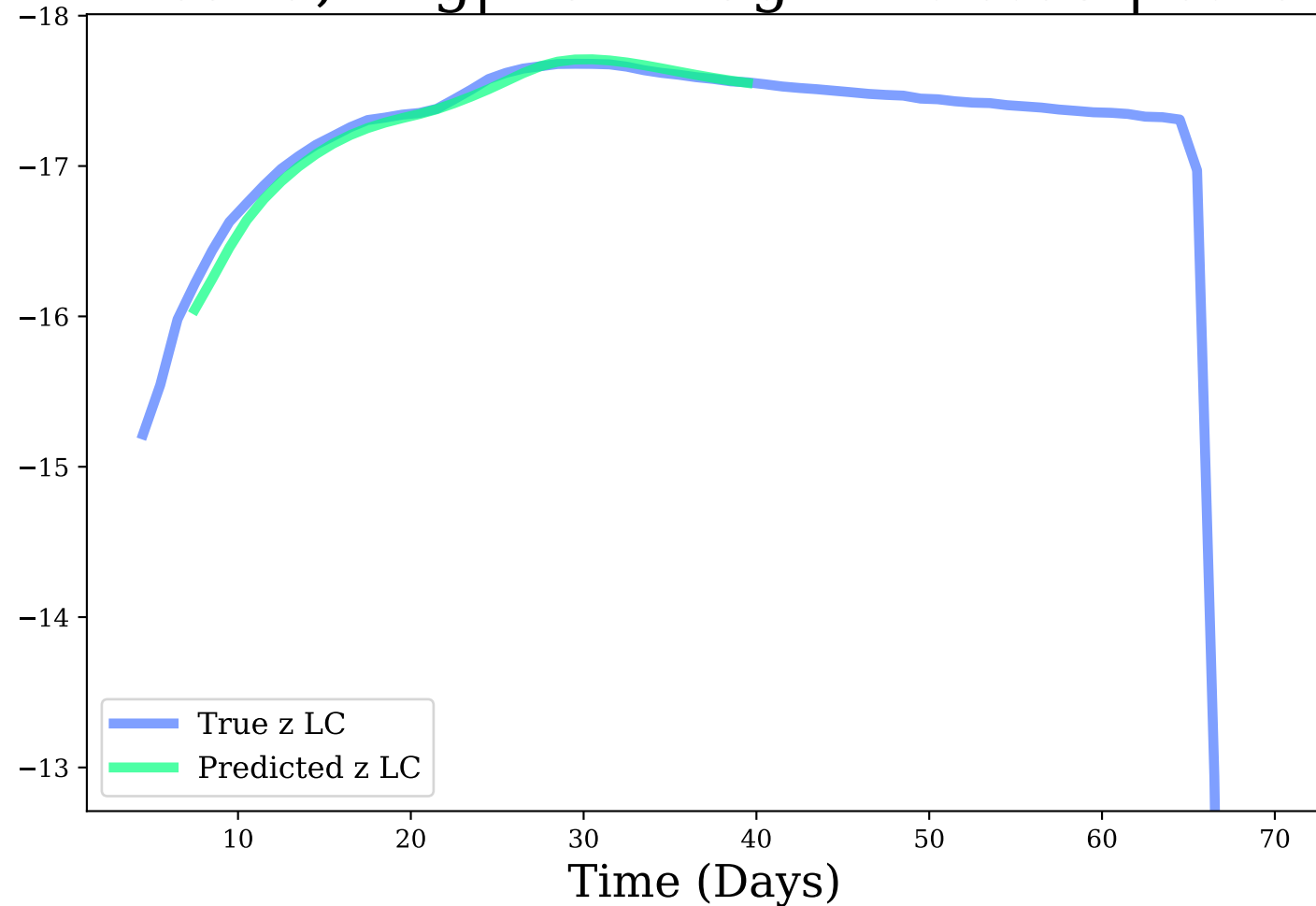
z-band, Avg|Max Mag Diff: 0.05 | 0.19
