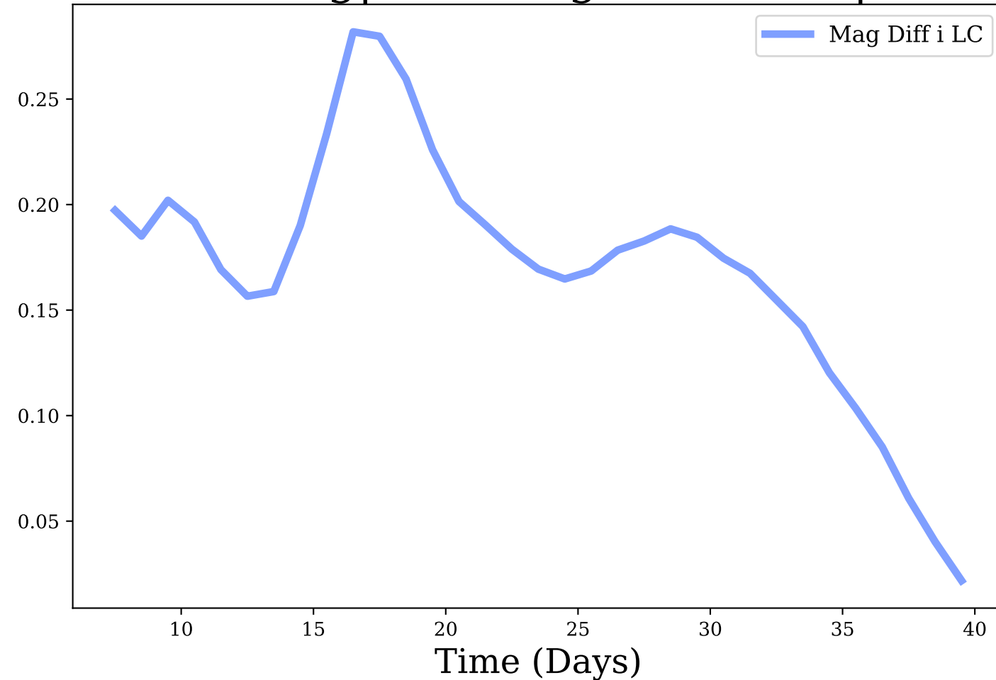
i-band, Avg|Max Mag Diff: 0.17 | 0.28
