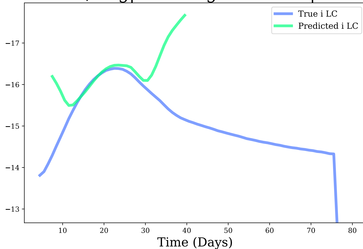
i-band, Avg|Max Mag Diff: 0.65 | 2.51
