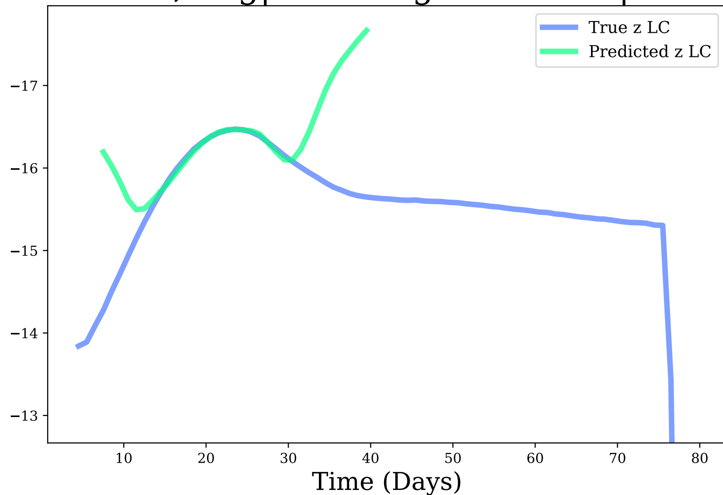
z-band, Avg|Max Mag Diff: 0.53 | 2.02
