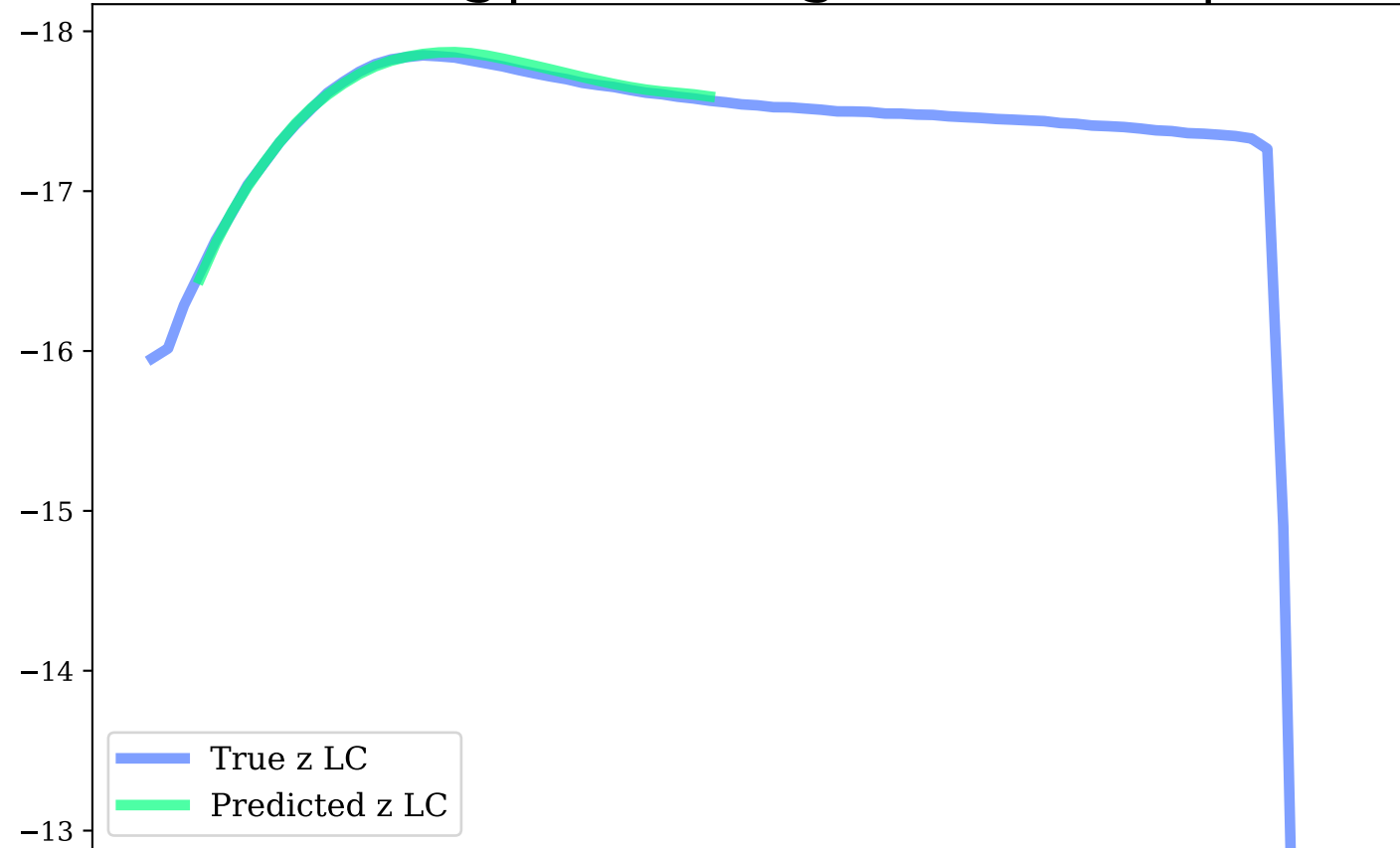
z-band, Avg|Max Mag Diff: 0.02 | 0.05
