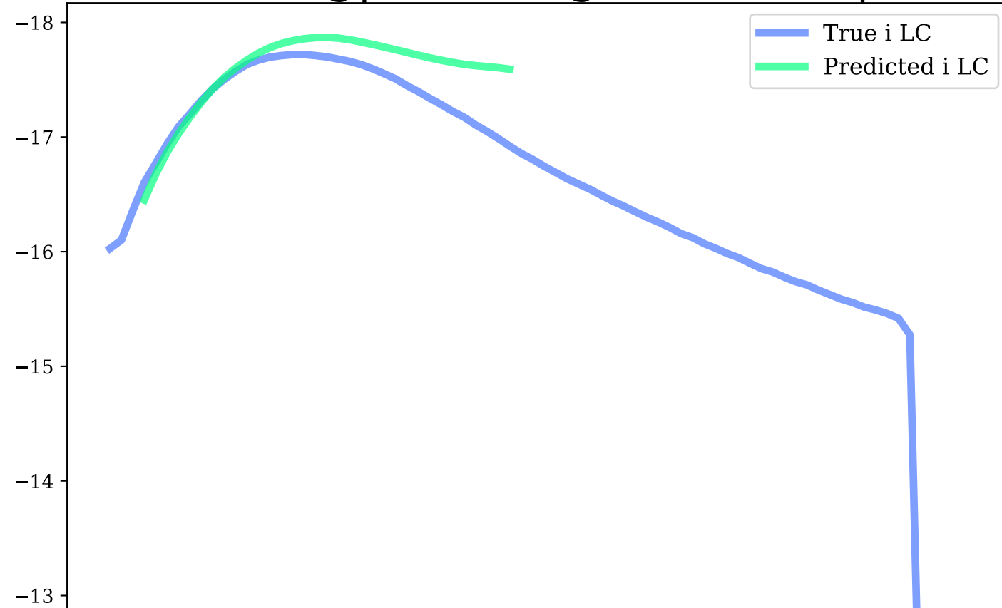
i-band, Avg|Max Mag Diff: 0.22 | 0.67
