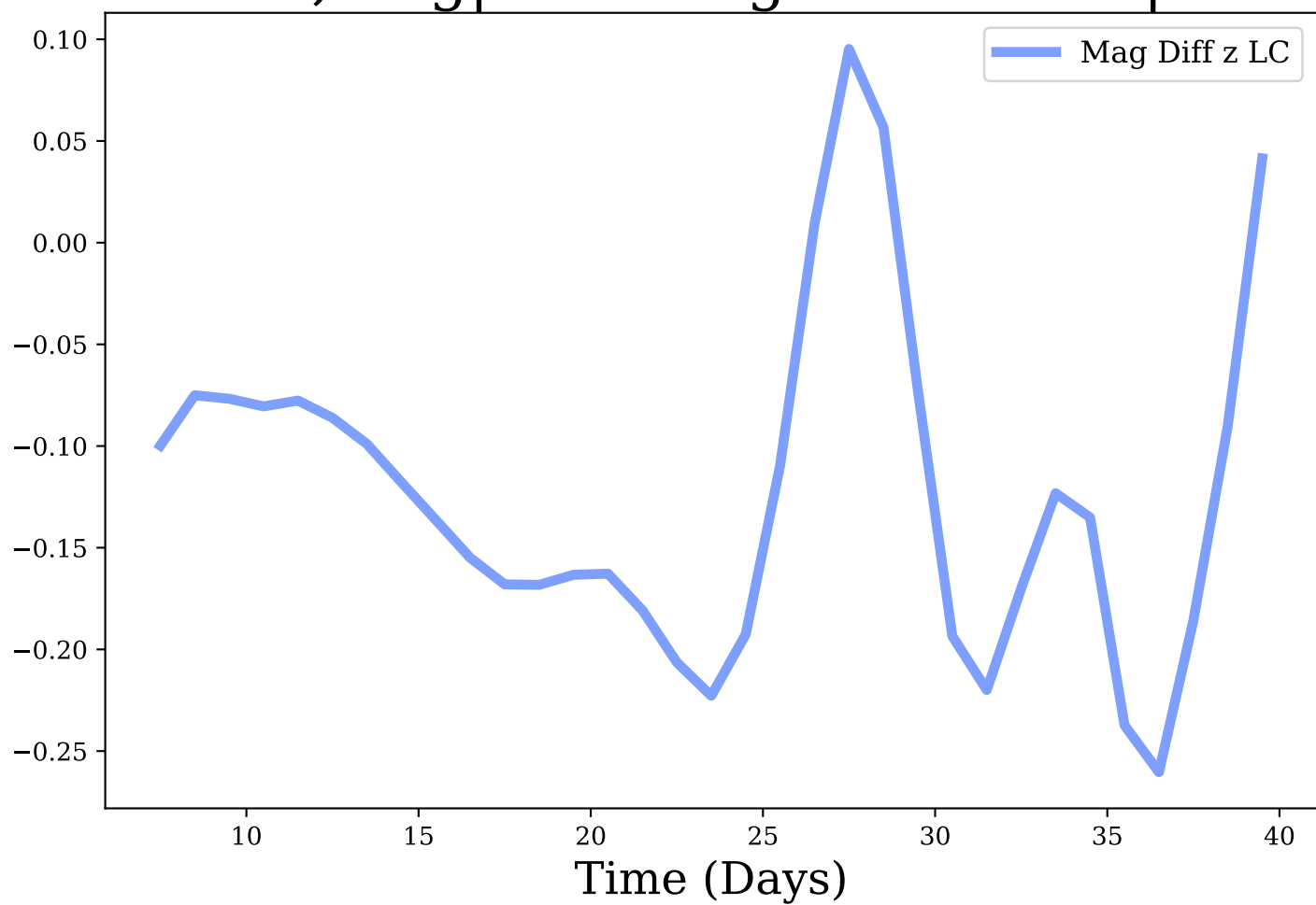
z-band, Avg|Max Mag Diff: -0.12 | 0.26
