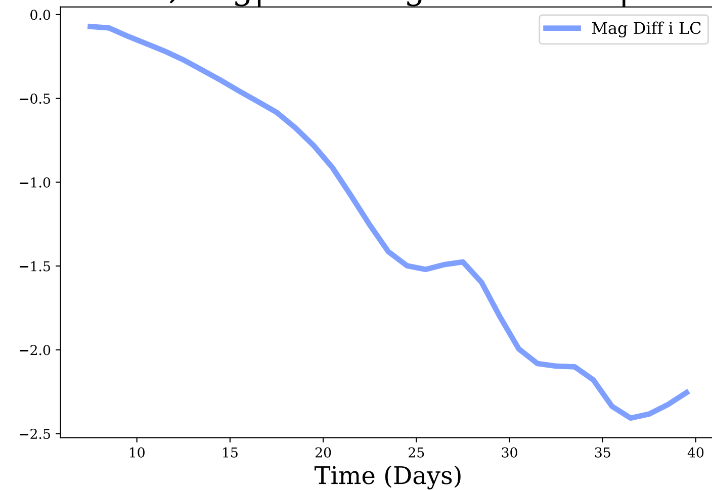
i-band, Avg|Max Mag Diff: -1.24 | 2.41
