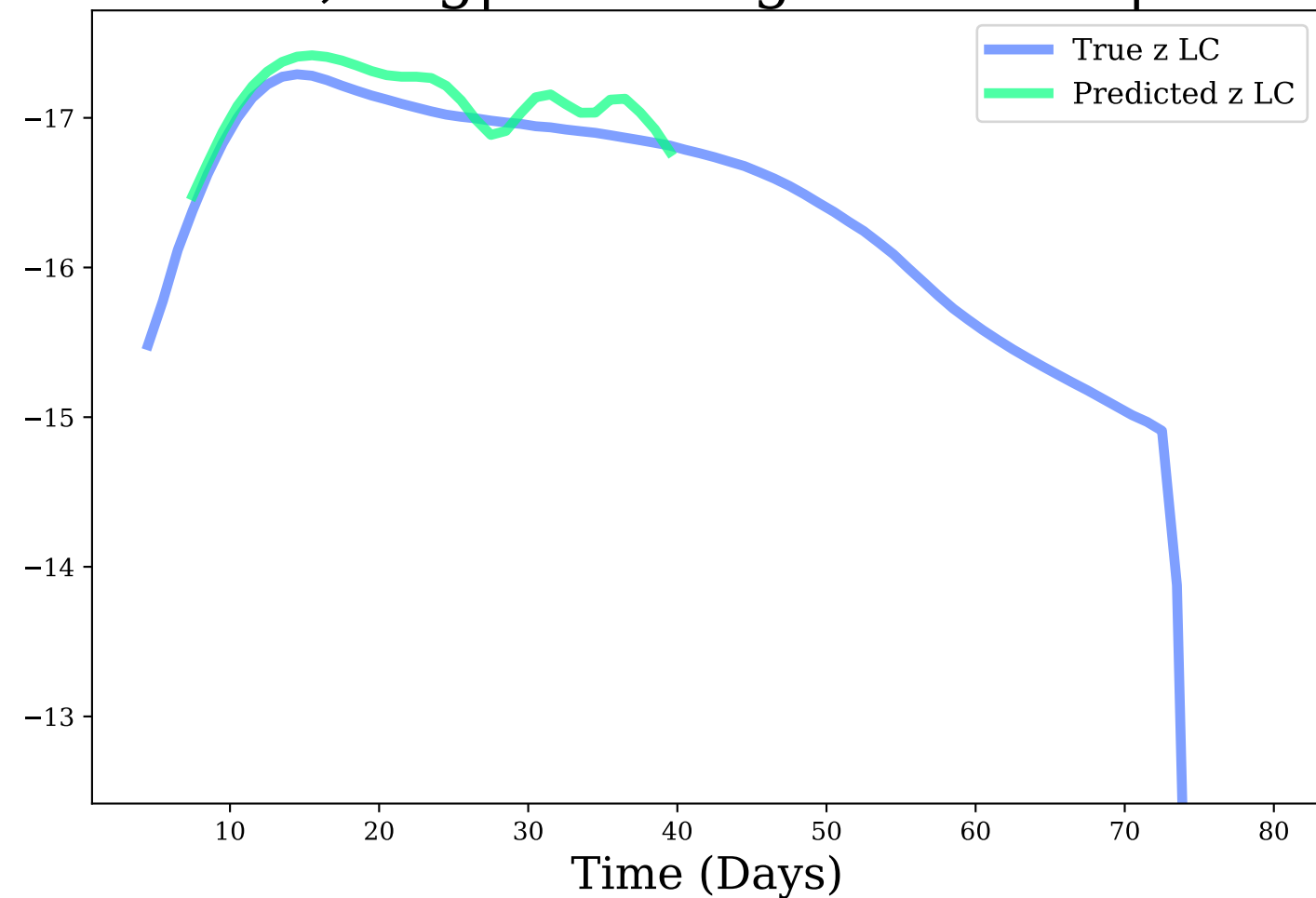
z-band, Avg|Max Mag Diff: 0.14 | 0.26
