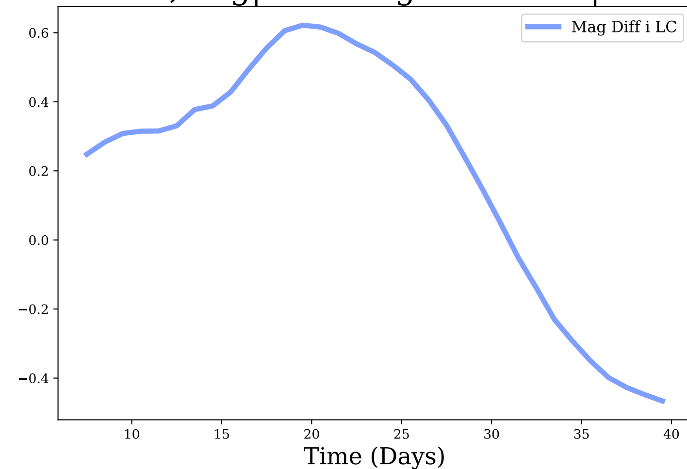
i-band, Avg|Max Mag Diff: 0.21 | 0.62
