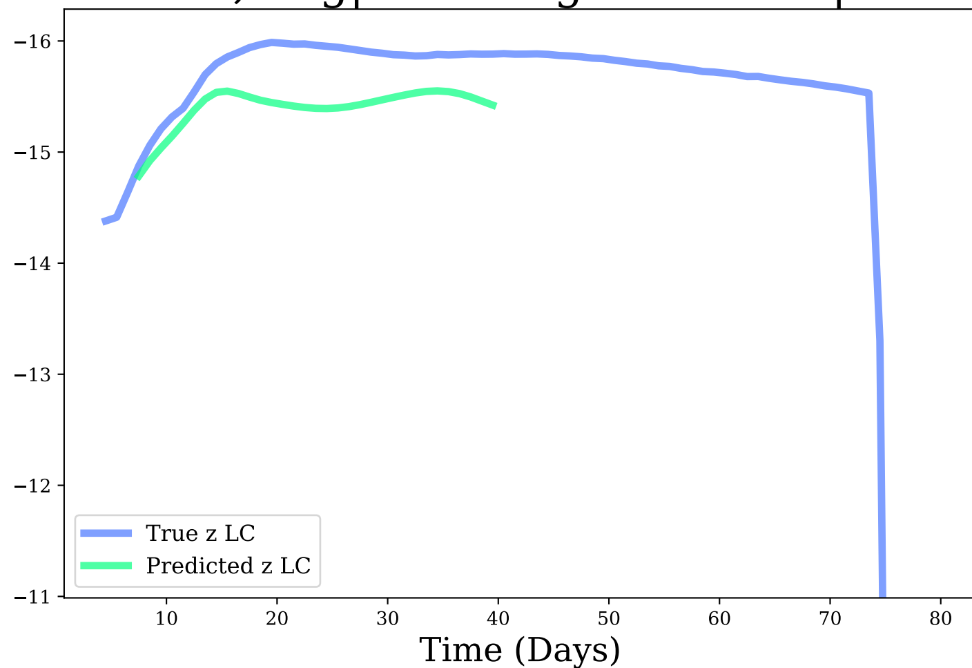
z-band, Avg|Max Mag Diff: 0.38 | 0.57
