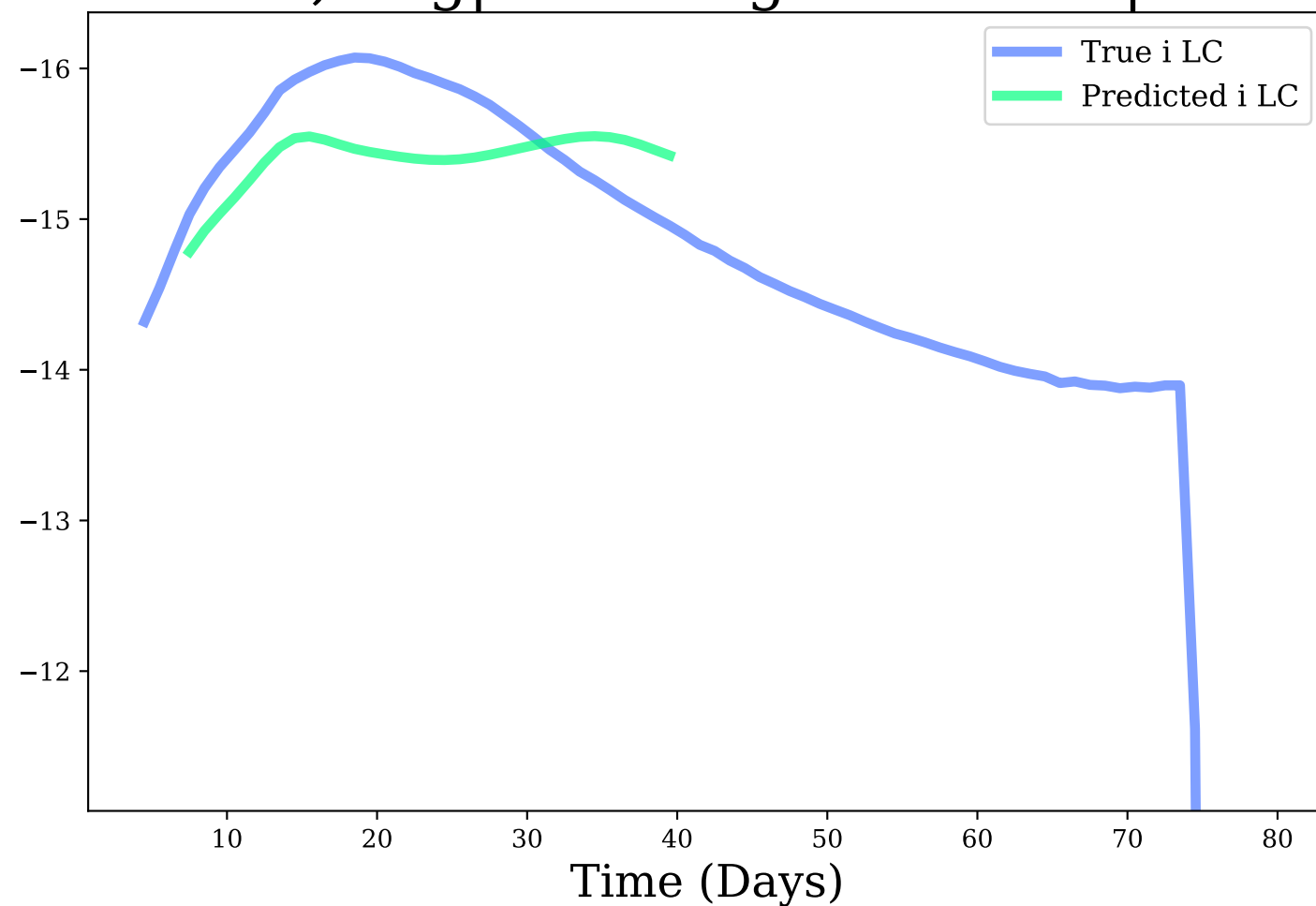
i-band, Avg|Max Mag Diff: 0.38 | 0.62
