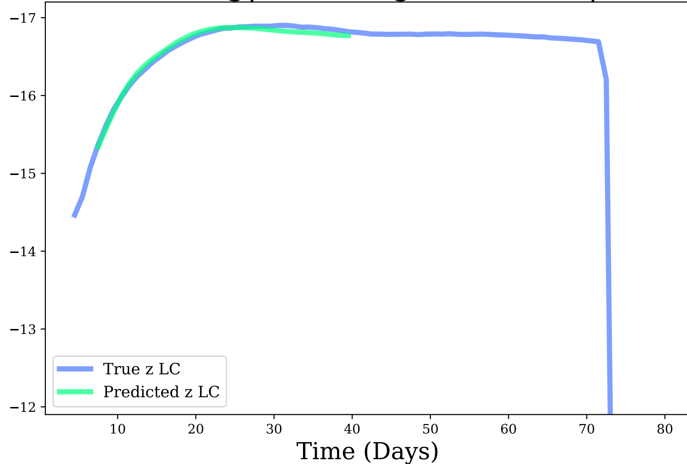
z-band, Avg|Max Mag Diff: 0.04 | 0.08
