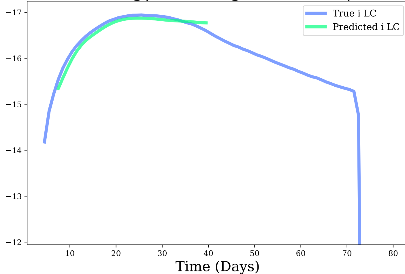
i-band, Avg|Max Mag Diff: 0.09 | 0.21
