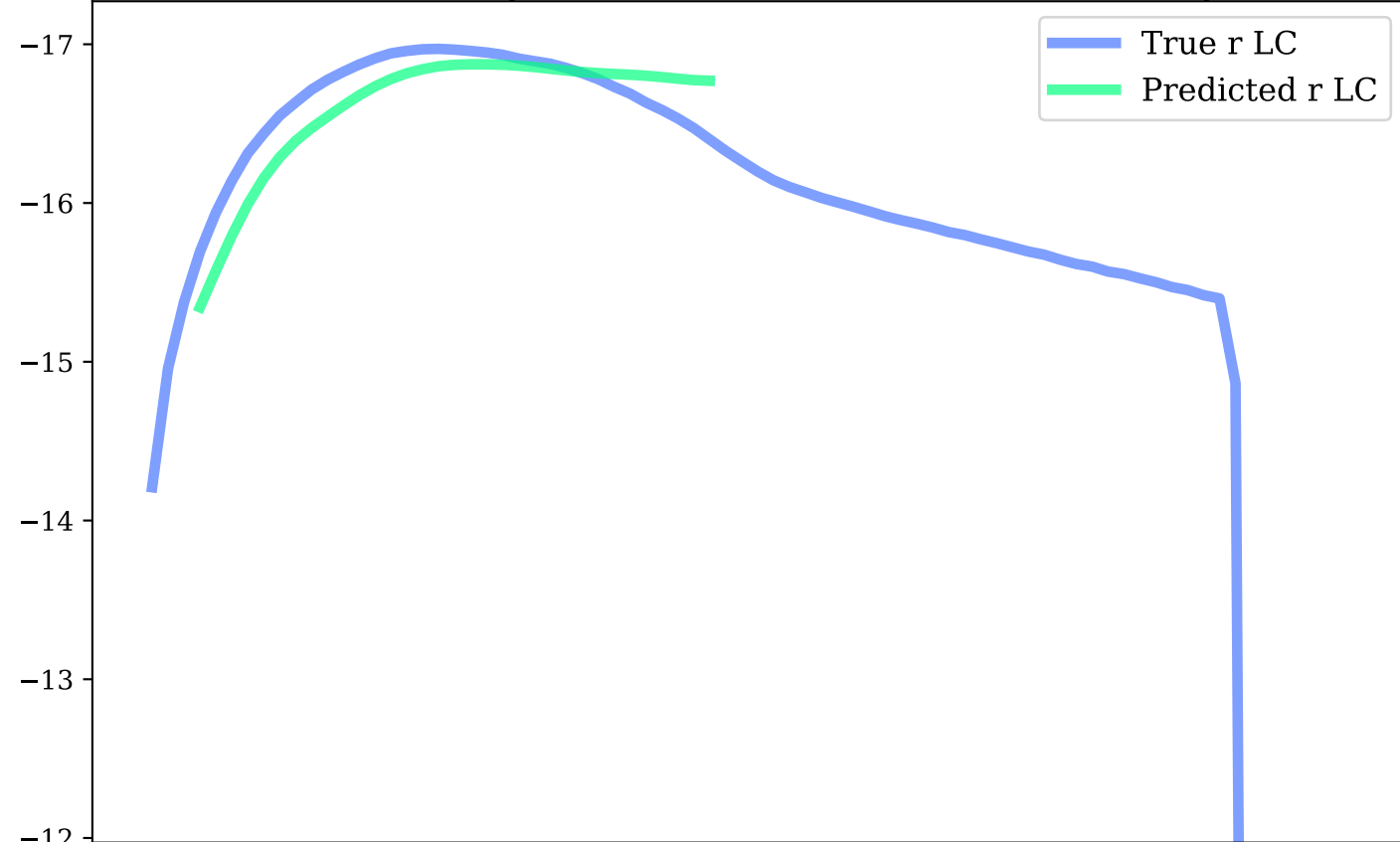
r-band, Avg|Max Mag Diff: 0.17 | 0.37
