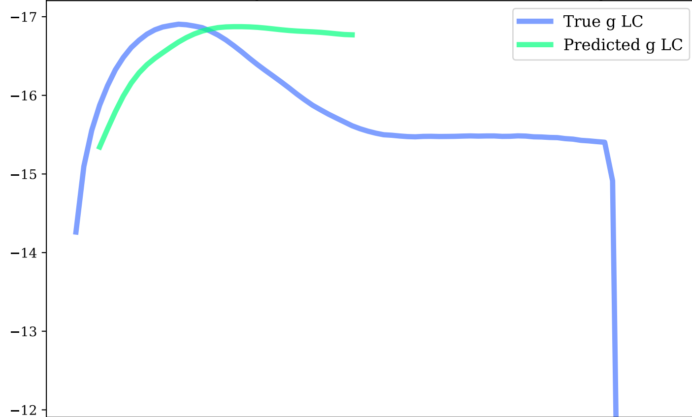
g-band, Avg|Max Mag Diff: 0.52 | 1.16
