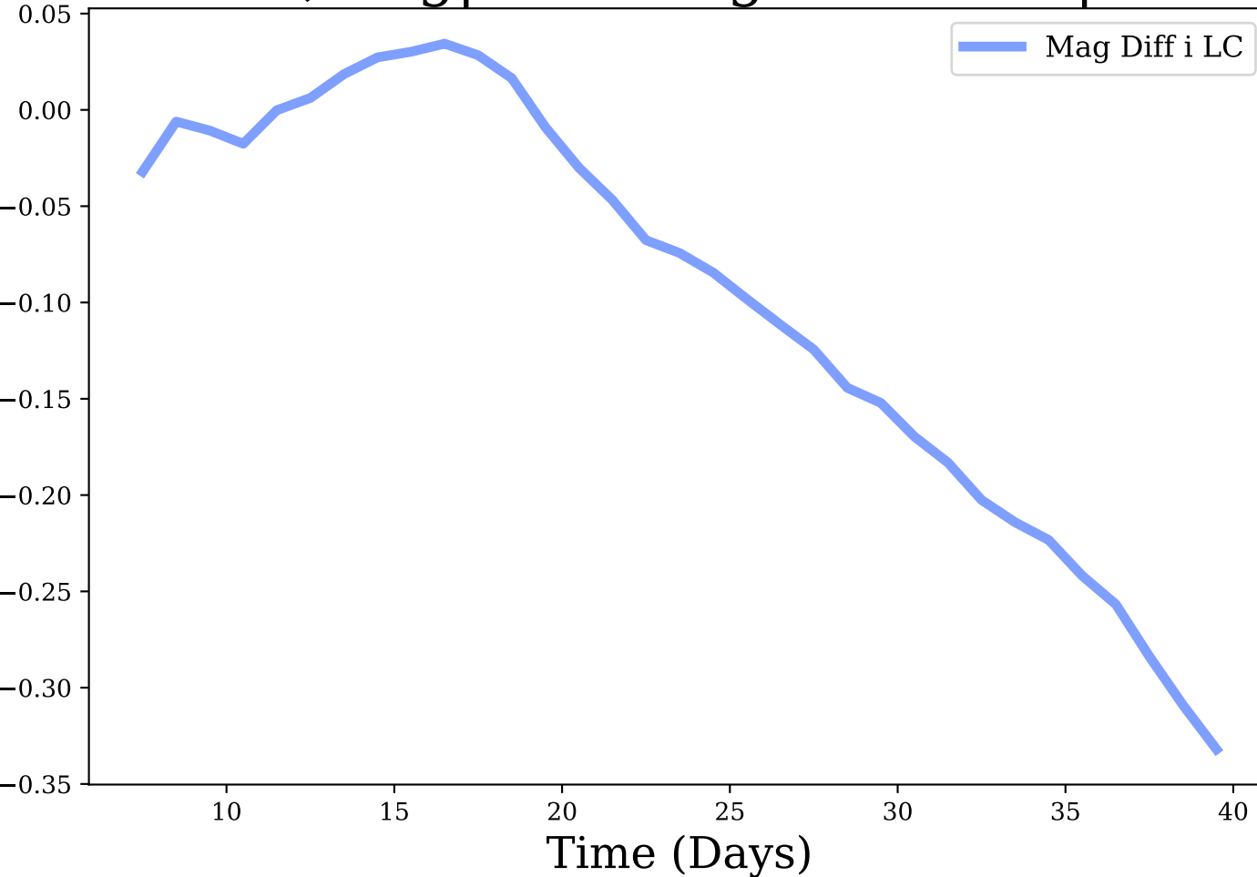
i-band, Avg|Max Mag Diff: -0.1 | 0.33
