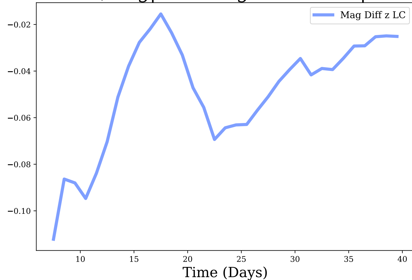
z-band, Avg|Max Mag Diff: -0.05 | 0.11
