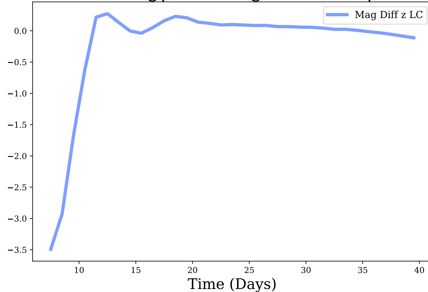
z-band, Avg|Max Mag Diff: -0.2 | 3.49
