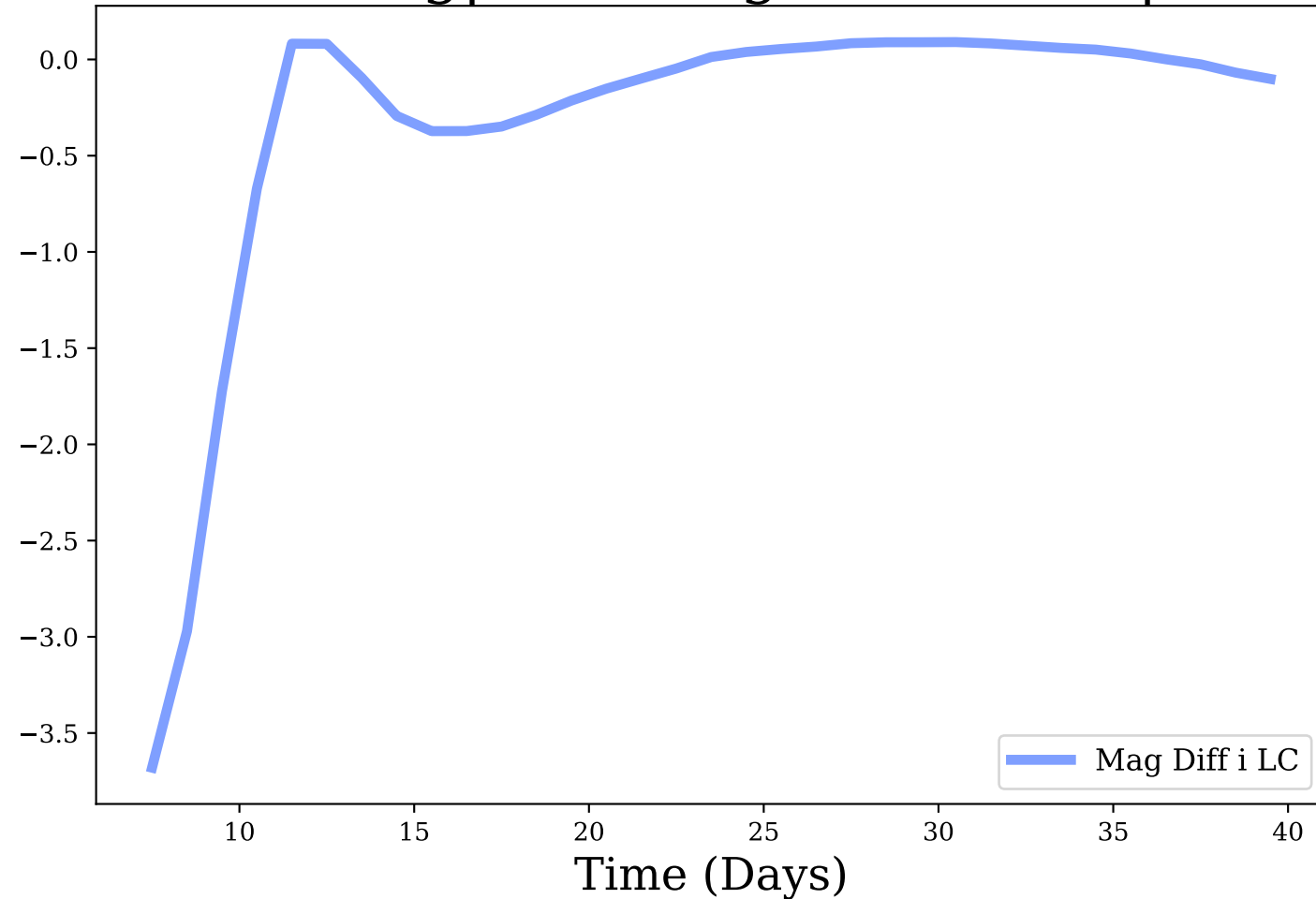
i-band, Avg|Max Mag Diff: -0.32 | 3.68
