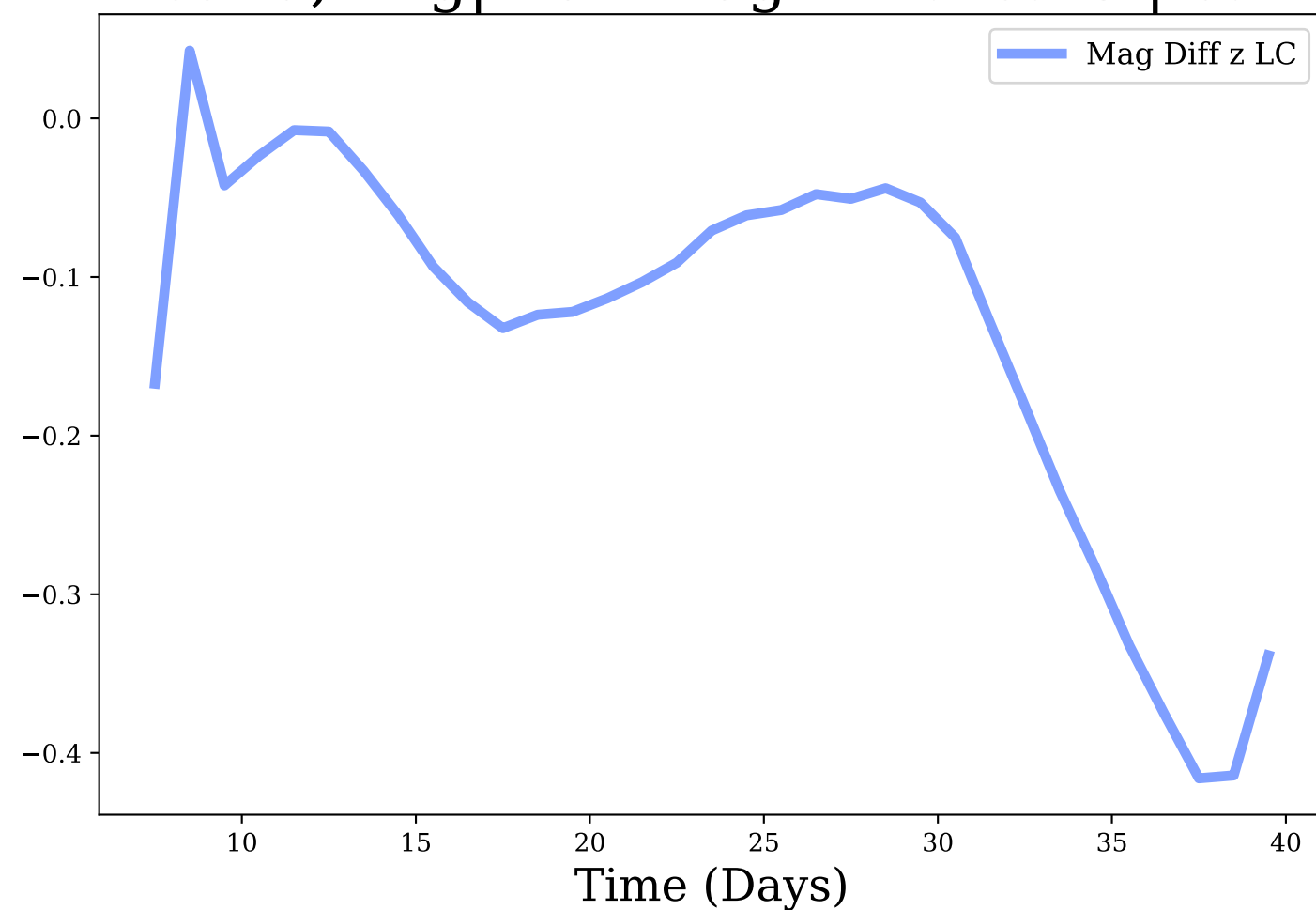
z-band, Avg|Max Mag Diff: -0.13 | 0.42
