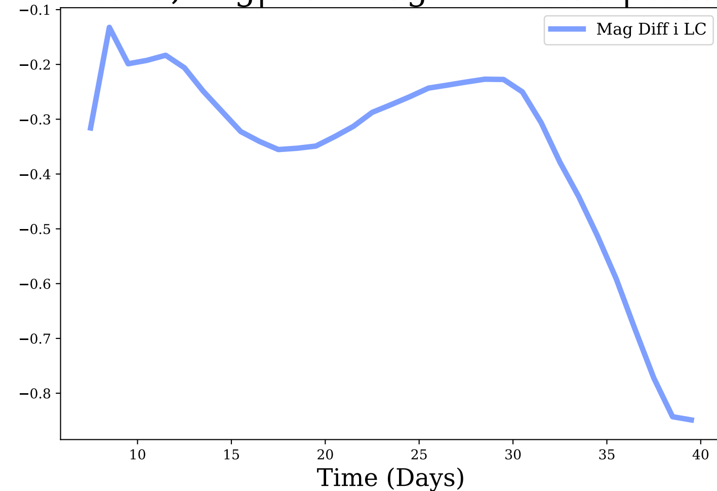
i-band, Avg|Max Mag Diff: -0.36 | 0.85
