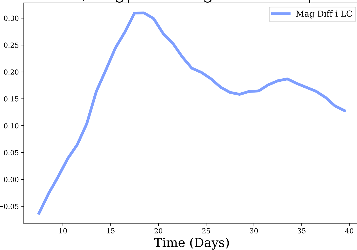
i-band, Avg|Max Mag Diff: 0.17 | 0.31
