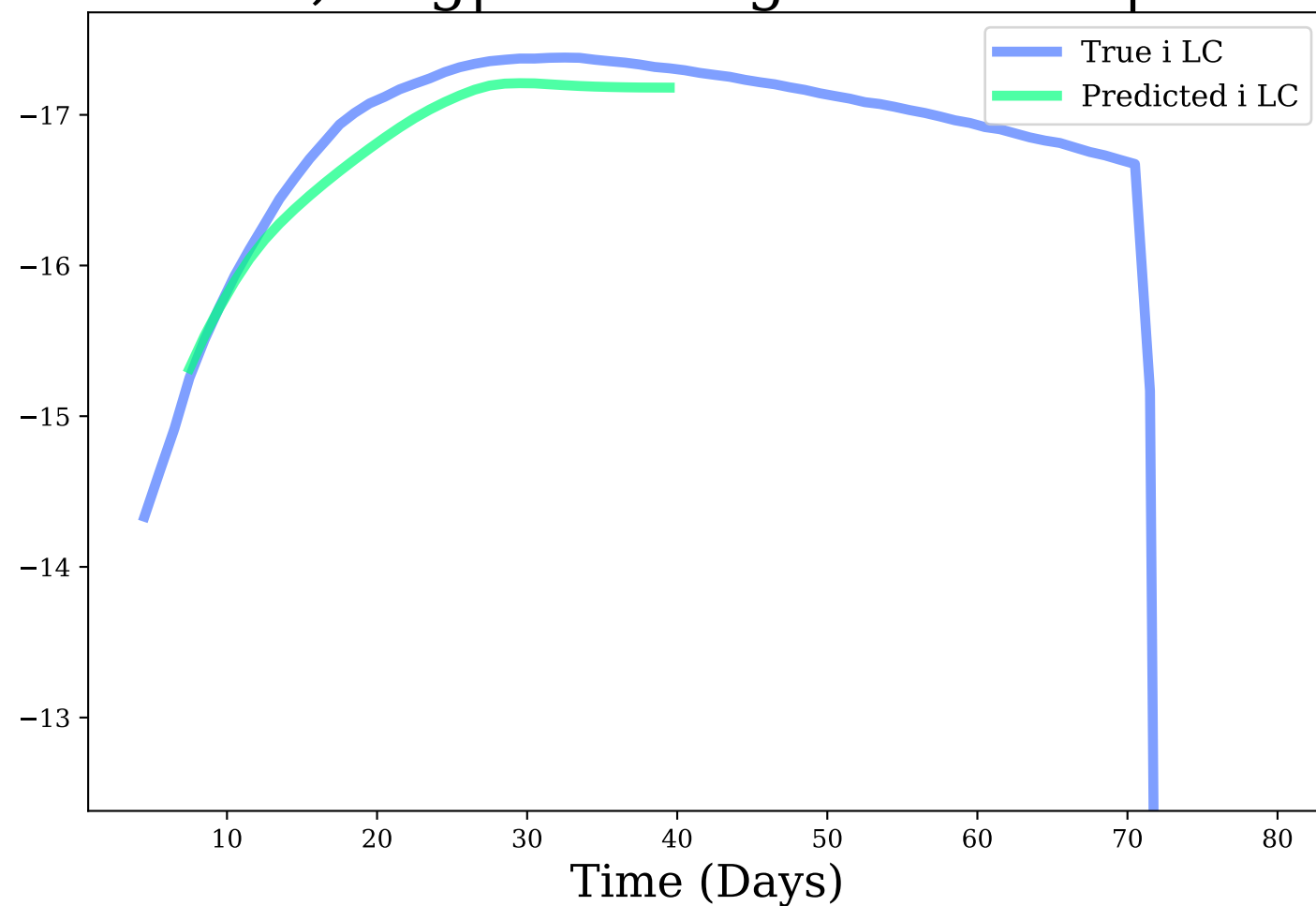
i-band, Avg|Max Mag Diff: 0.17 | 0.31
