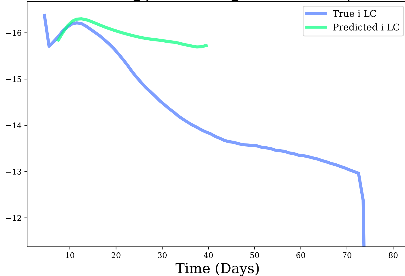
i-band, Avg|Max Mag Diff: 0.84 | 1.87
