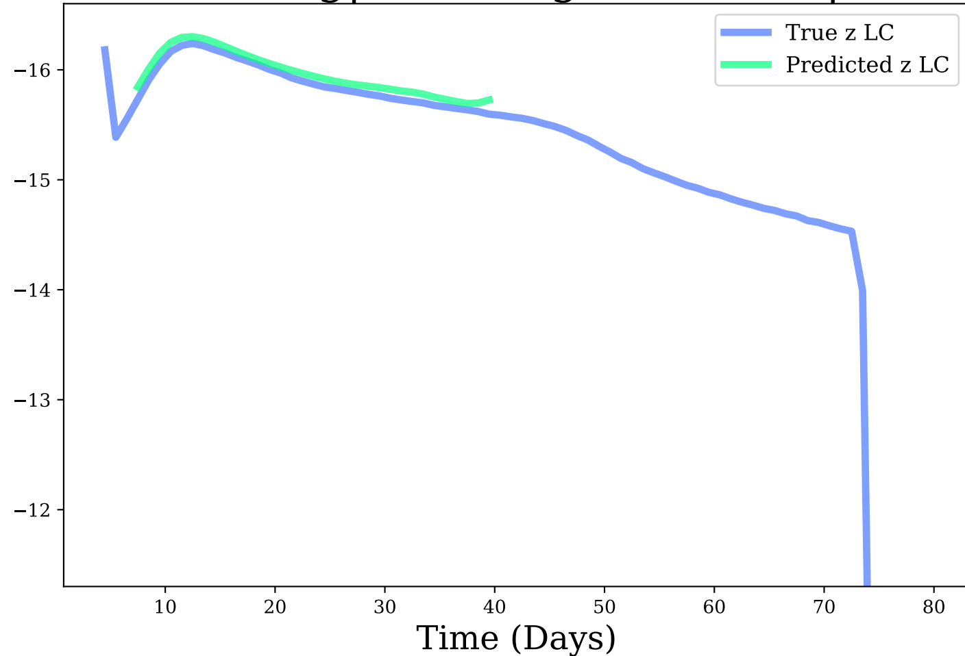
z-band, Avg|Max Mag Diff: 0.07 | 0.13
