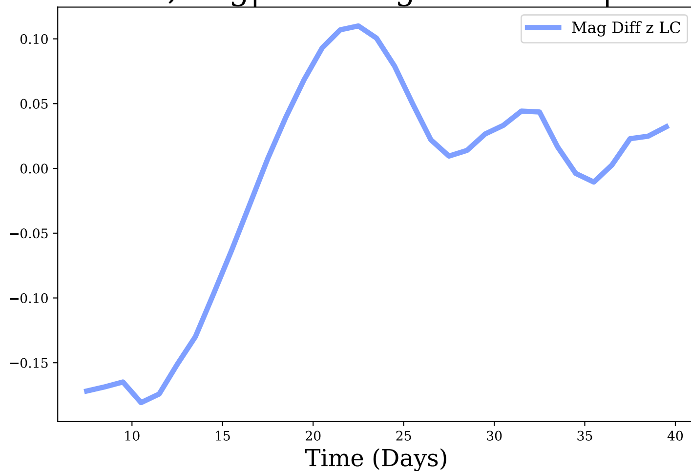
z-band, Avg|Max Mag Diff: -0.01 | 0.18
