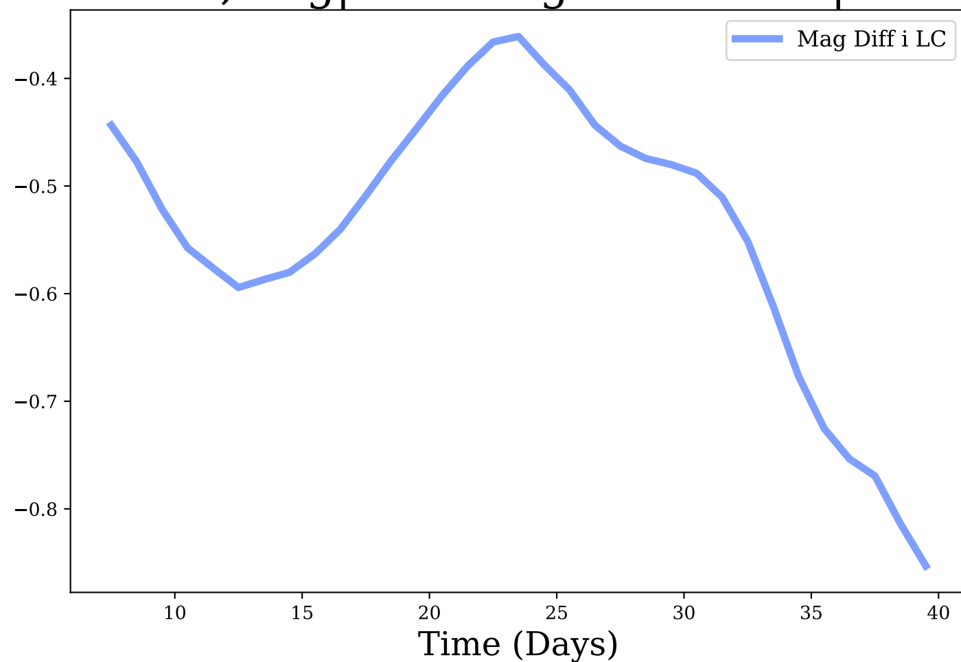
i-band, Avg|Max Mag Diff: -0.54 | 0.85
