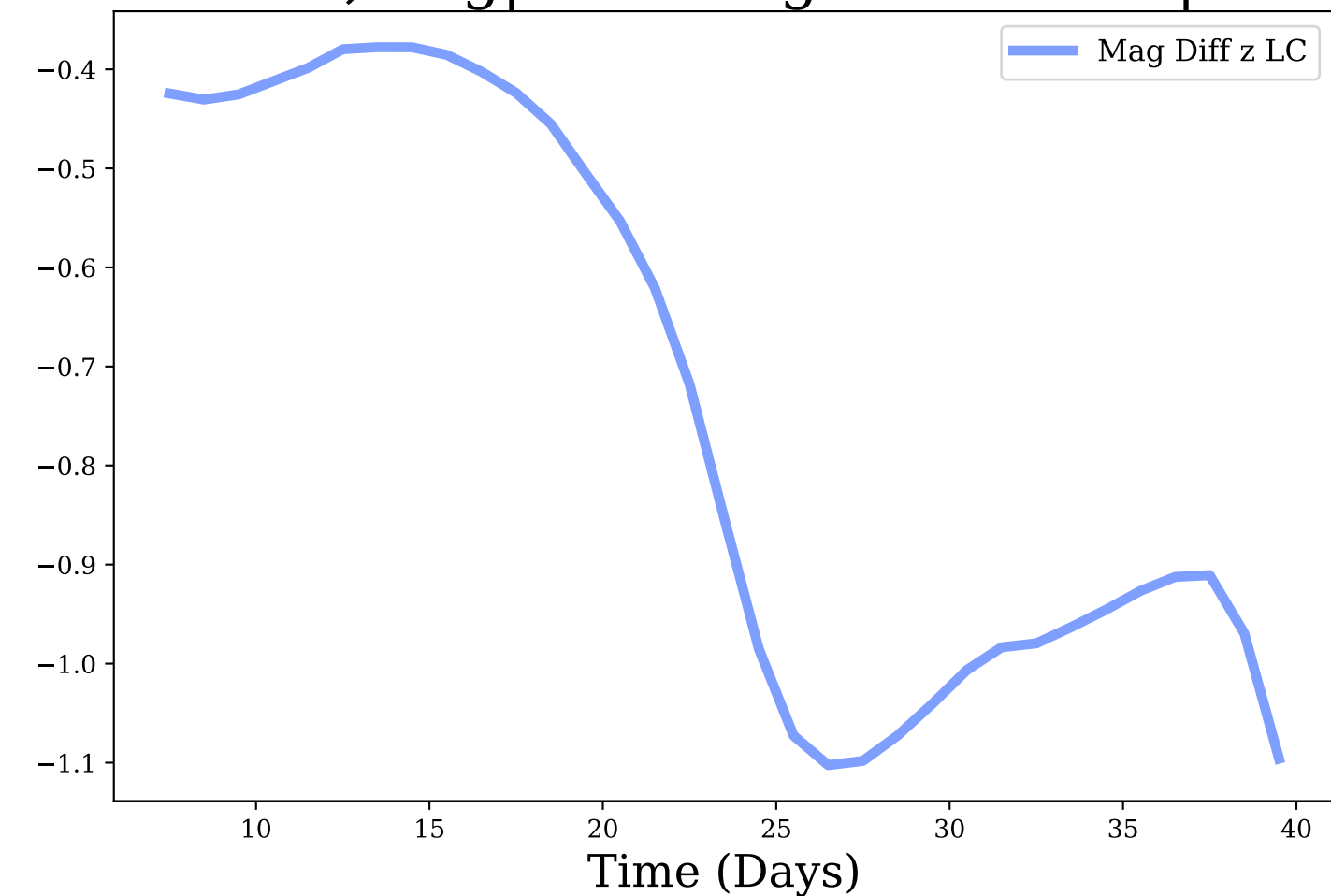
z-band, Avg|Max Mag Diff: -0.73 | 1.1
