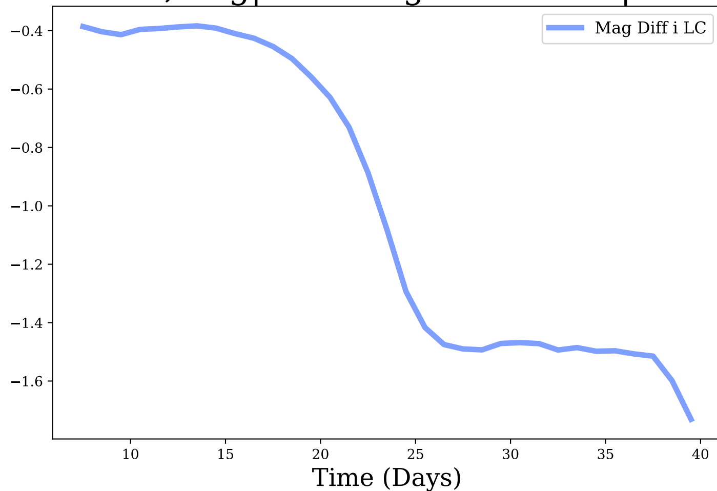
i-band, Avg|Max Mag Diff: -0.99 | 1.73
