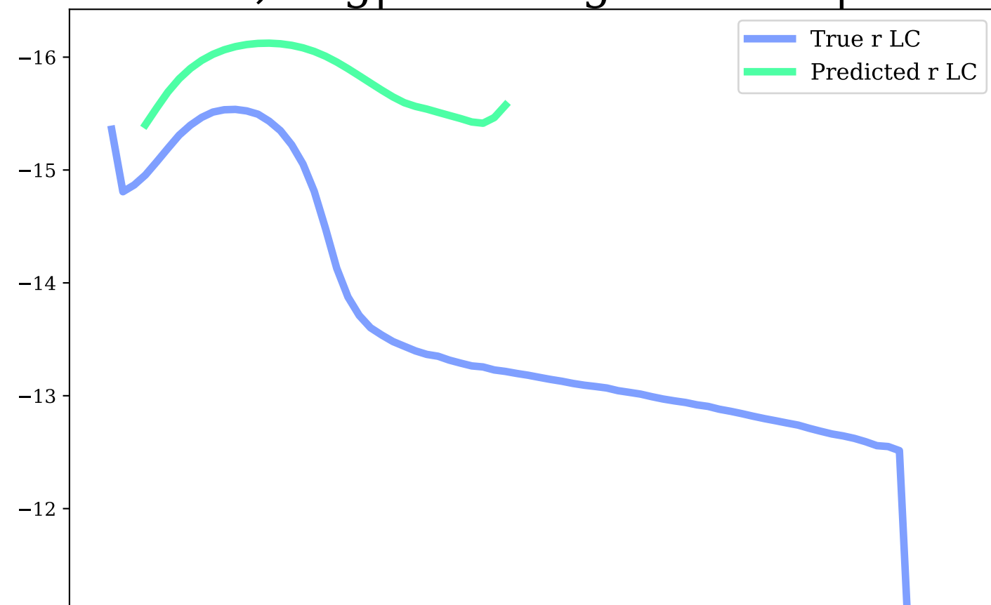
z-band, Avg|Max Mag Diff: 0.73 | 1.1
