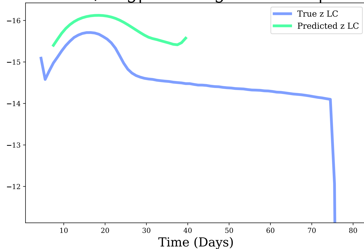
z-band, Avg|Max Mag Diff: 0.73 | 1.1
