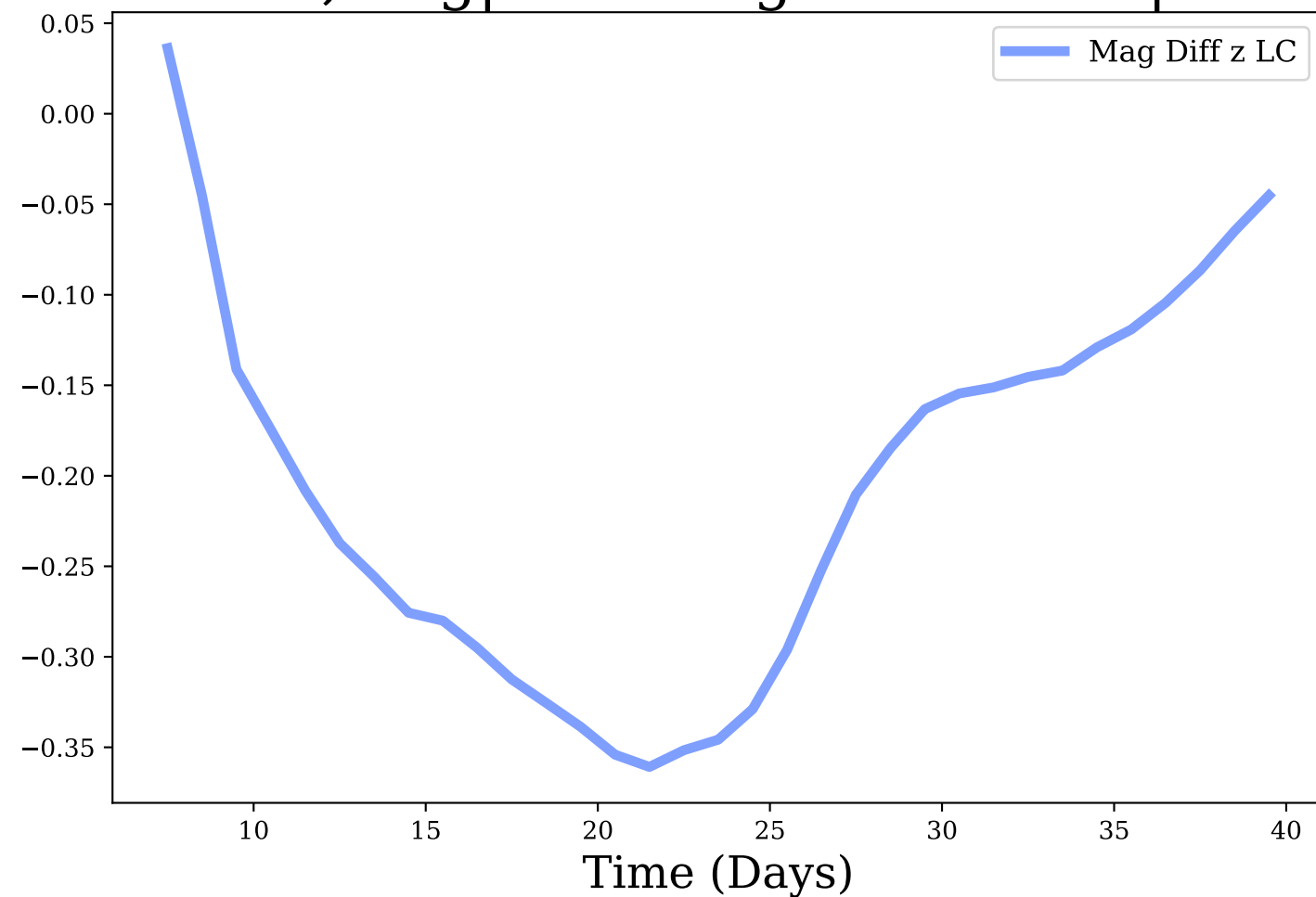
z-band, Avg|Max Mag Diff: -0.21 | 0.36
