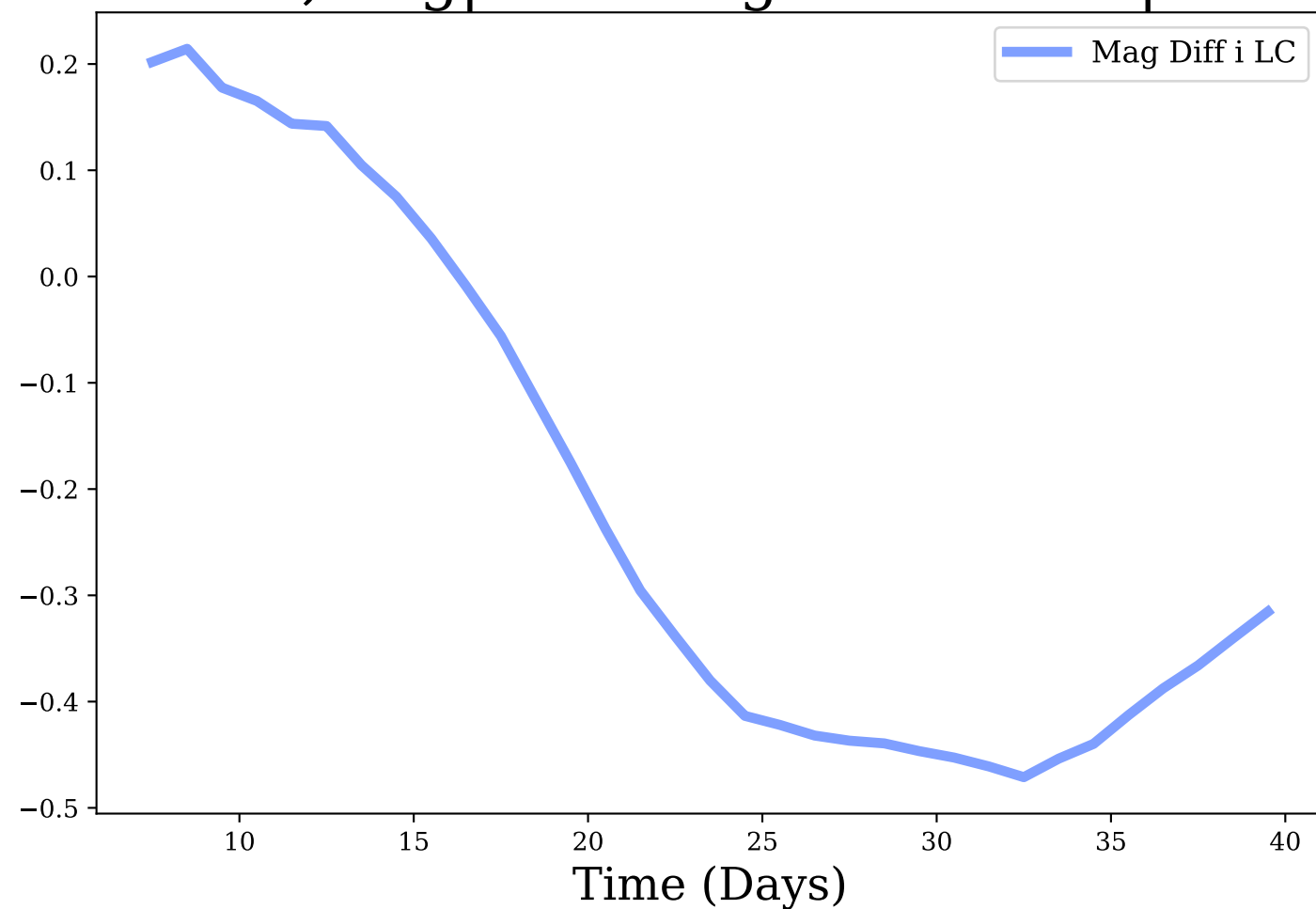
i-band, Avg|Max Mag Diff: -0.21 | 0.47
