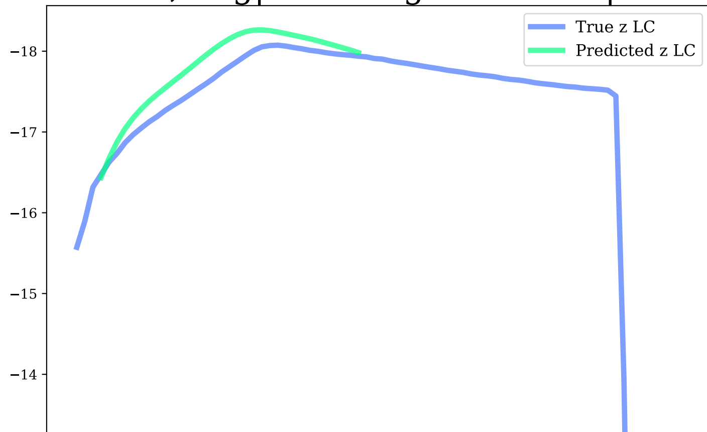
z-band, Avg|Max Mag Diff: 0.21 | 0.36
