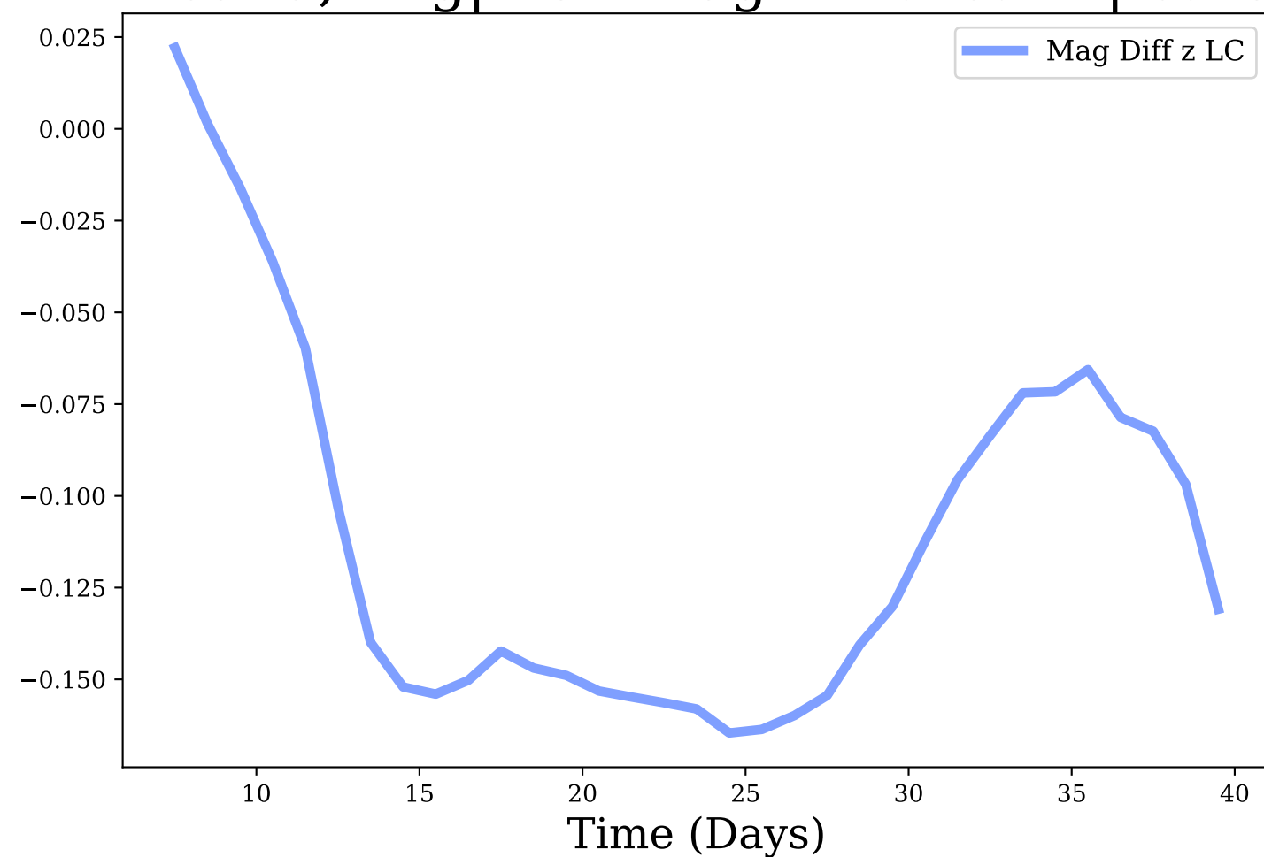
z-band, Avg|Max Mag Diff: -0.11 | 0.16
