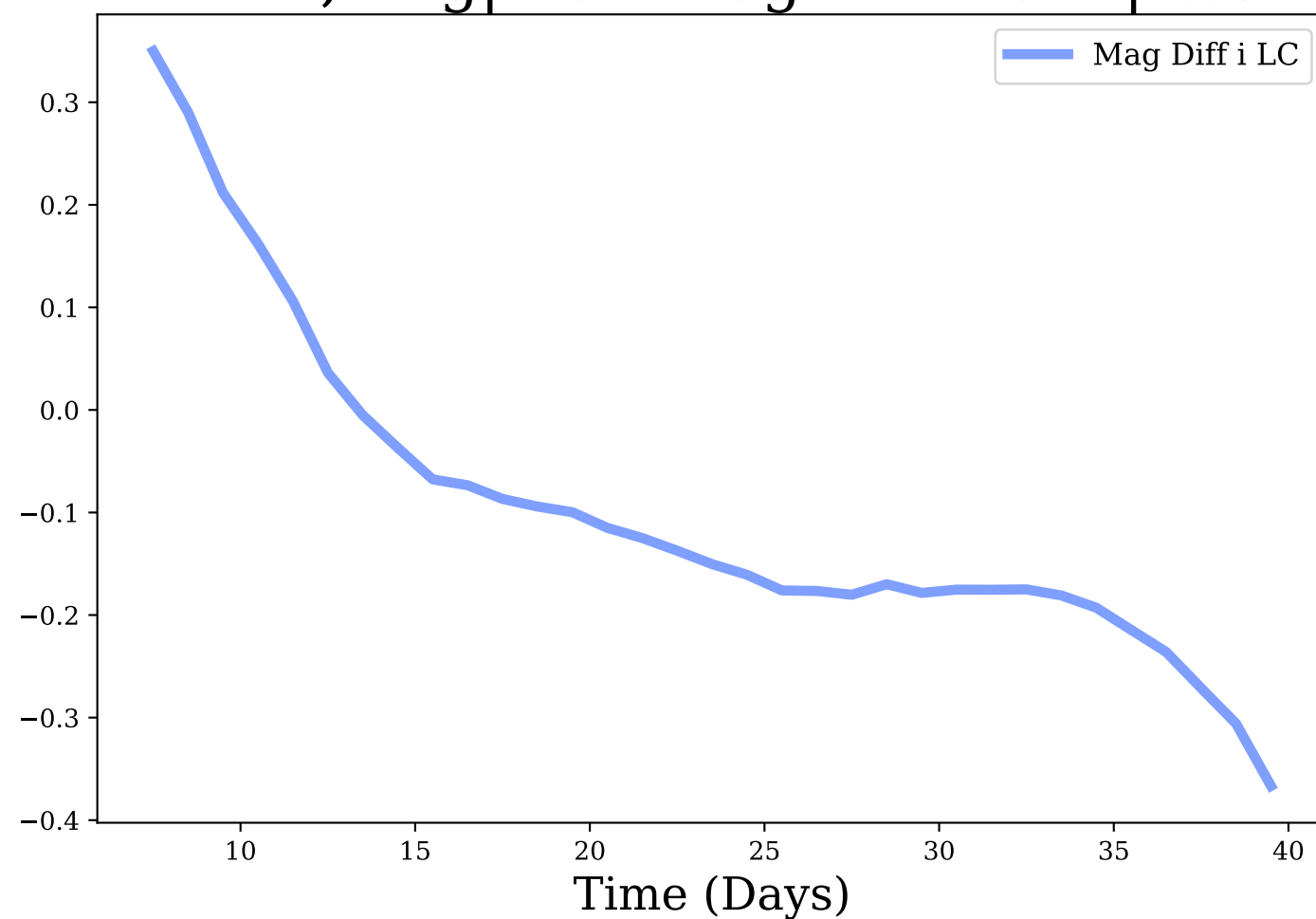
i-band, Avg|Max Mag Diff: -0.1 | 0.37
