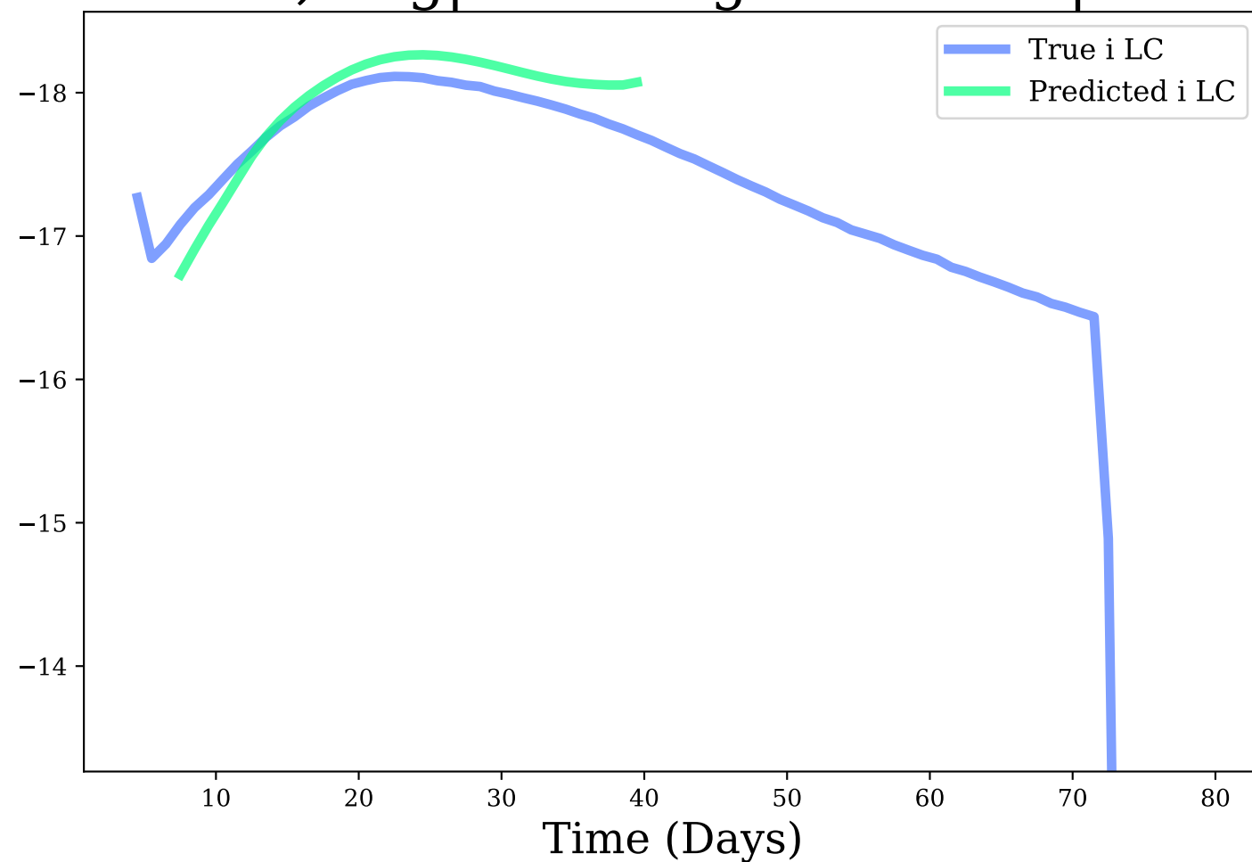
i-band, Avg|Max Mag Diff: 0.17 | 0.37
