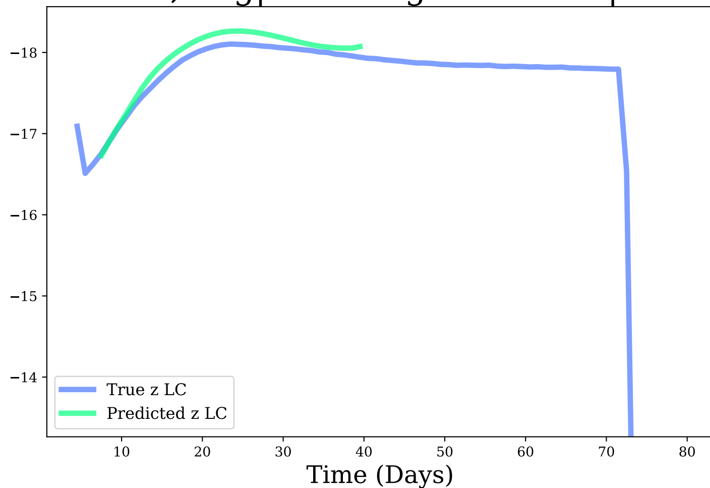
z-band, Avg|Max Mag Diff: 0.11 | 0.16
