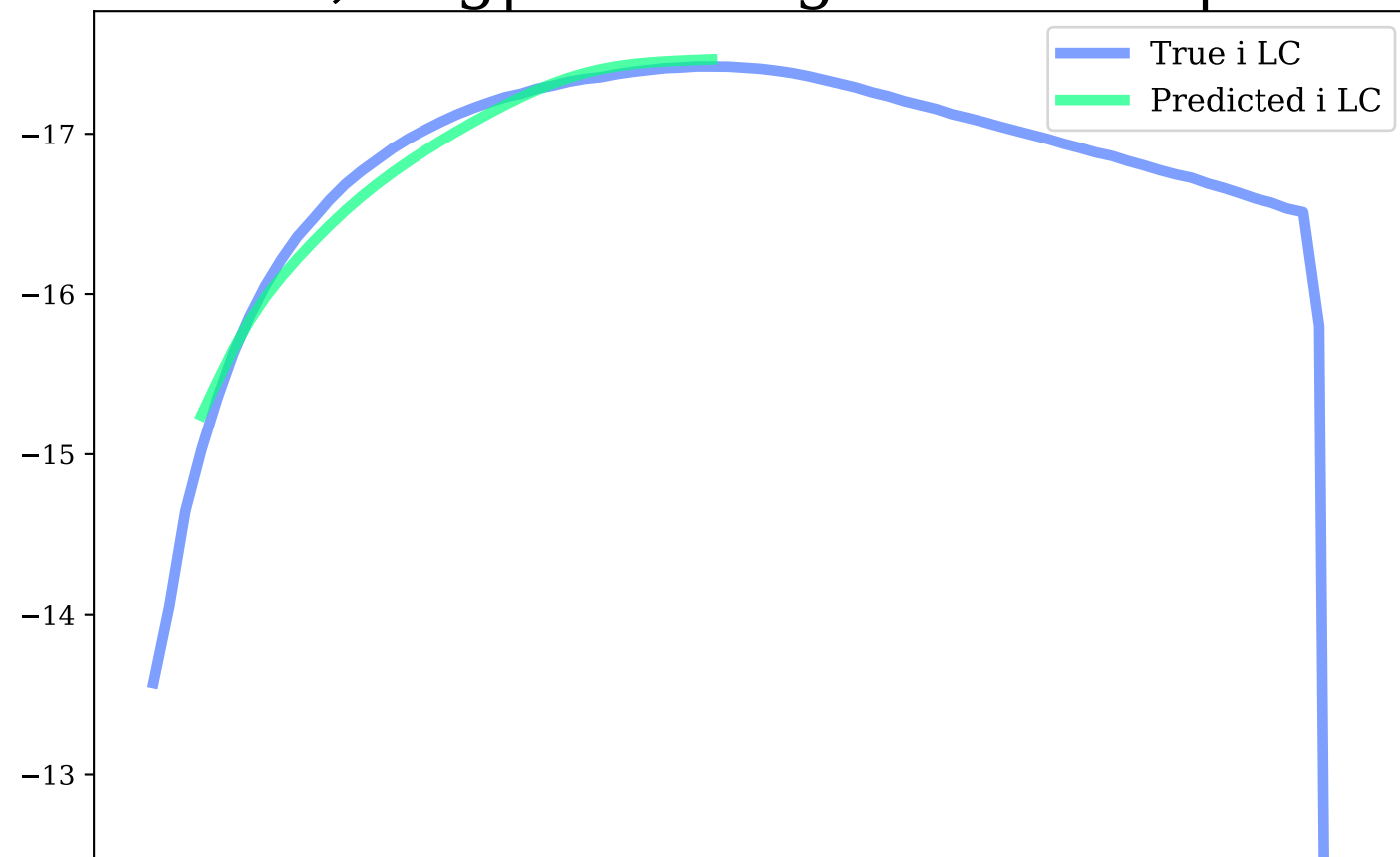
i-band, Avg|Max Mag Diff: 0.08 | 0.22
