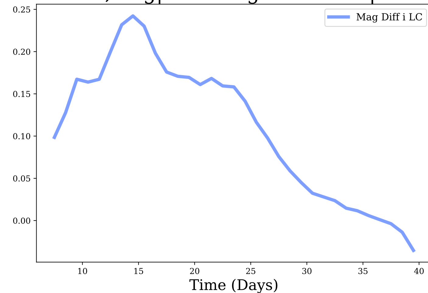
i-band, Avg|Max Mag Diff: 0.11 | 0.24
