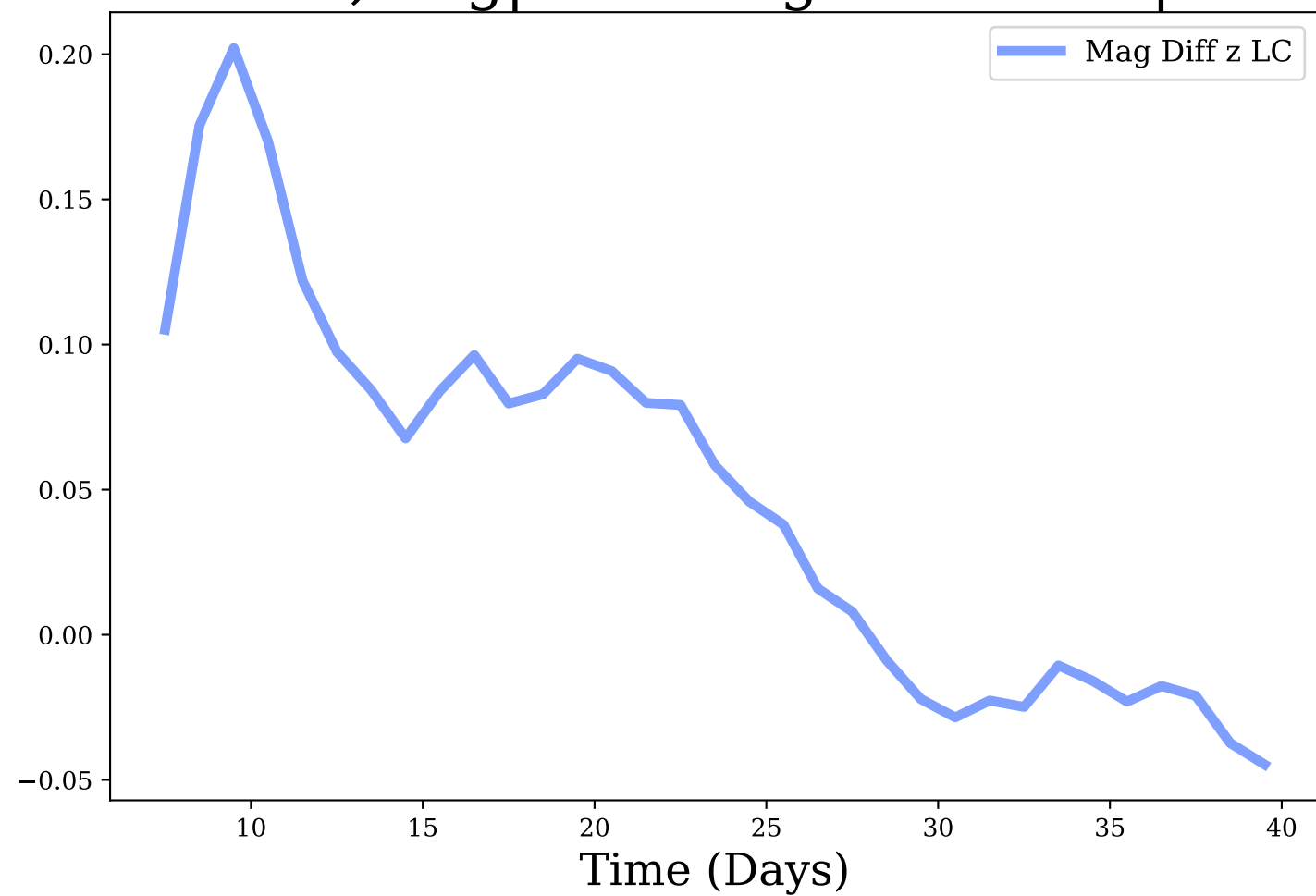
z-band, Avg|Max Mag Diff: 0.05 | 0.2
