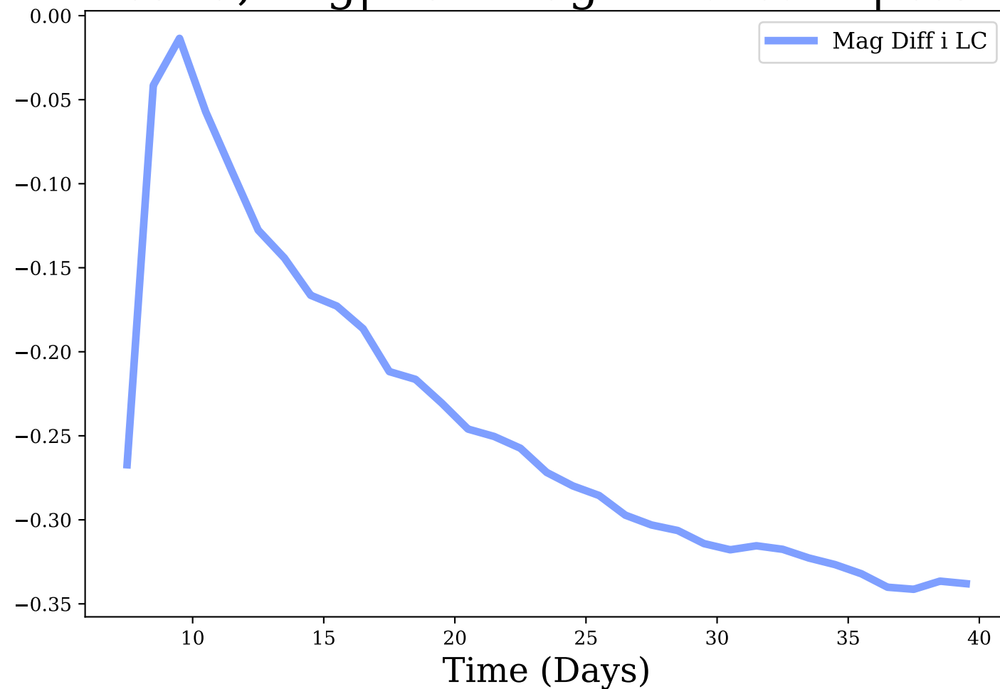
i-band, Avg|Max Mag Diff: -0.24 | 0.34
