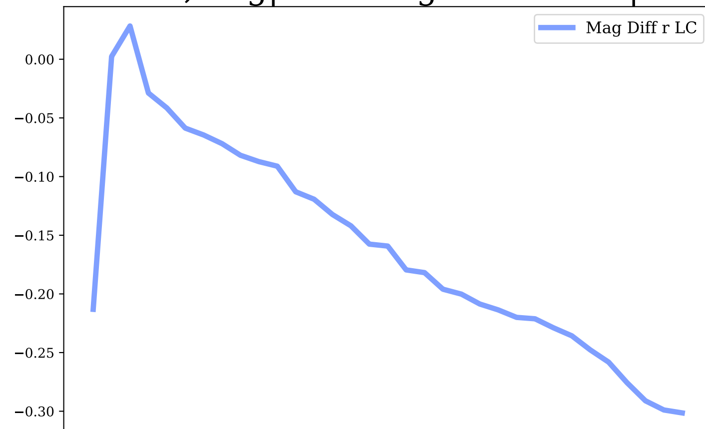
z-band, Avg|Max Mag Diff: -0.02 | 0.21
