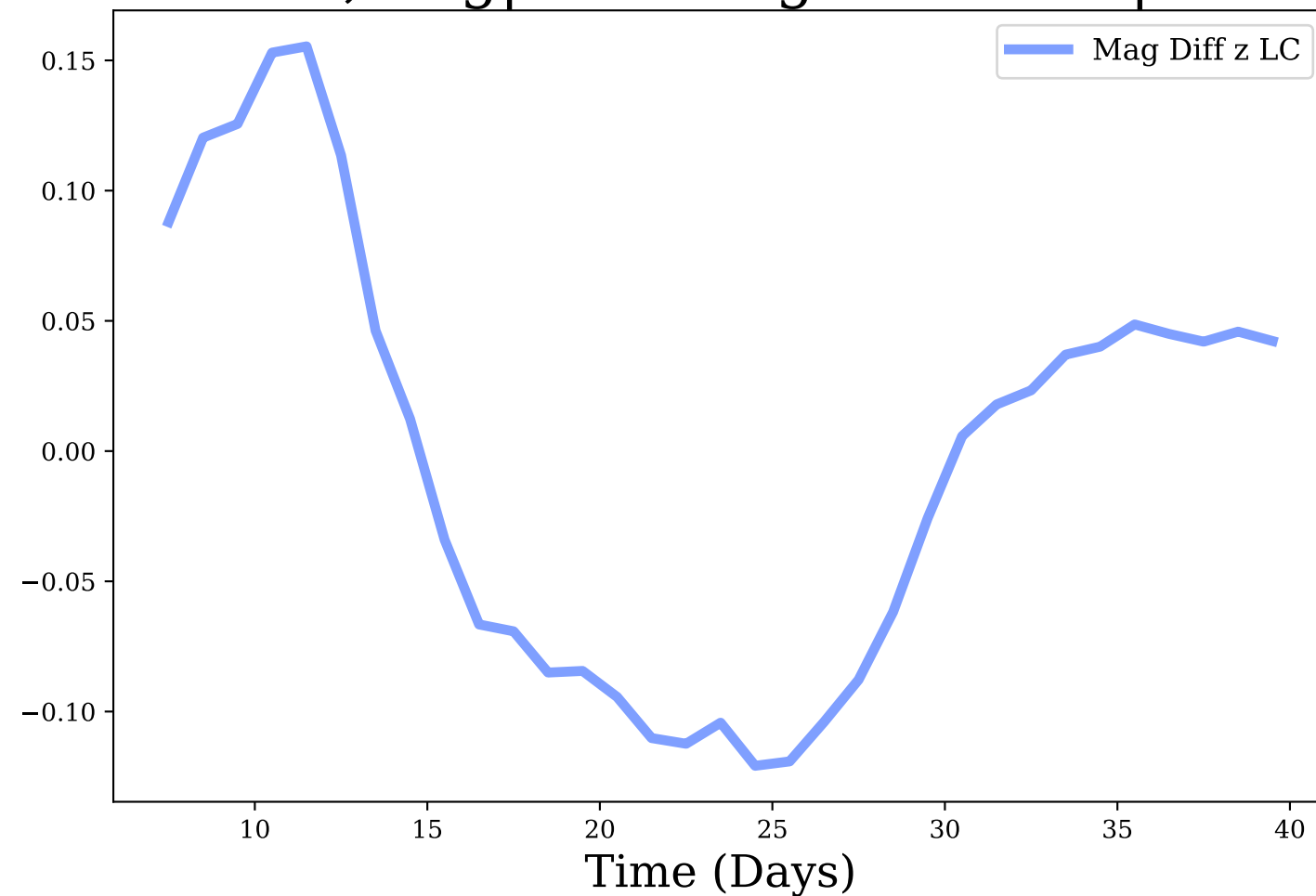
z-band, Avg|Max Mag Diff: -0.0 | 0.16
