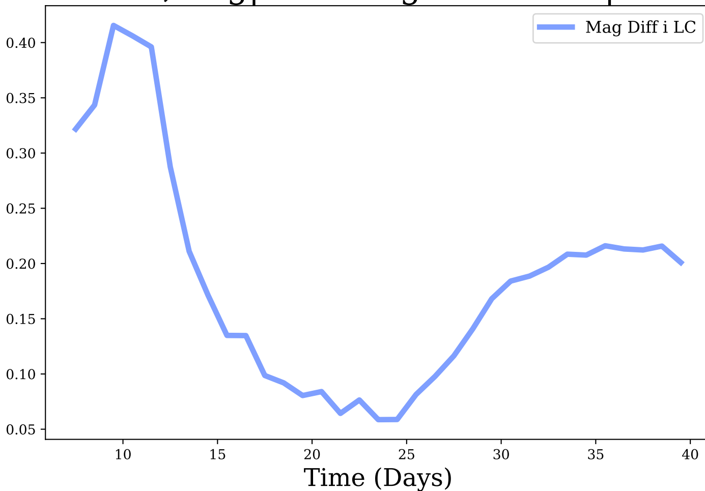
i-band, Avg|Max Mag Diff: 0.18 | 0.42
