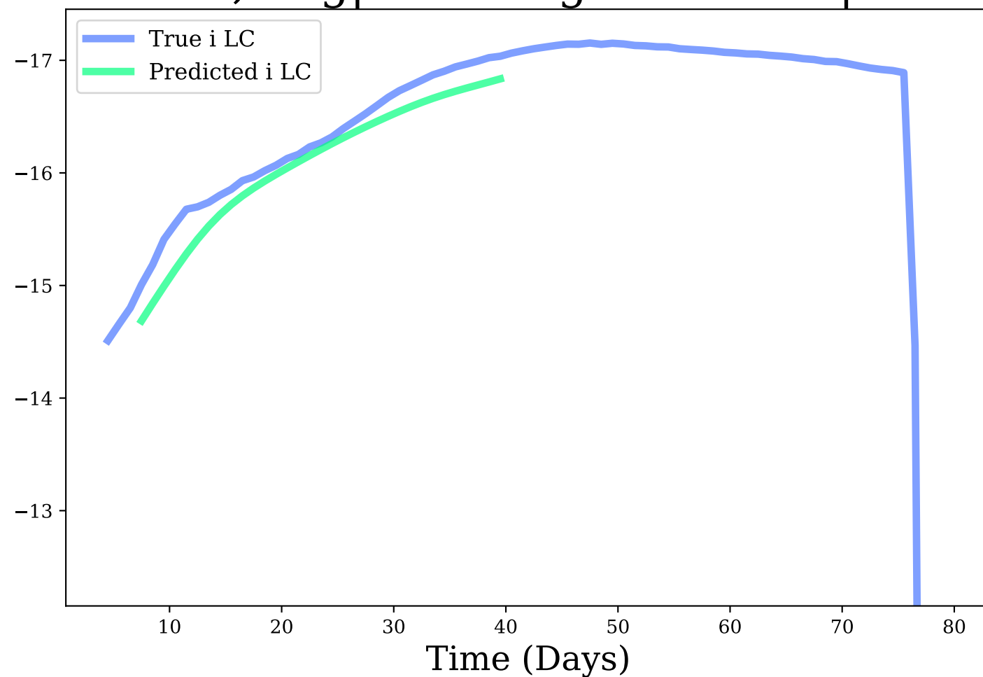
i-band, Avg|Max Mag Diff: 0.18 | 0.42
