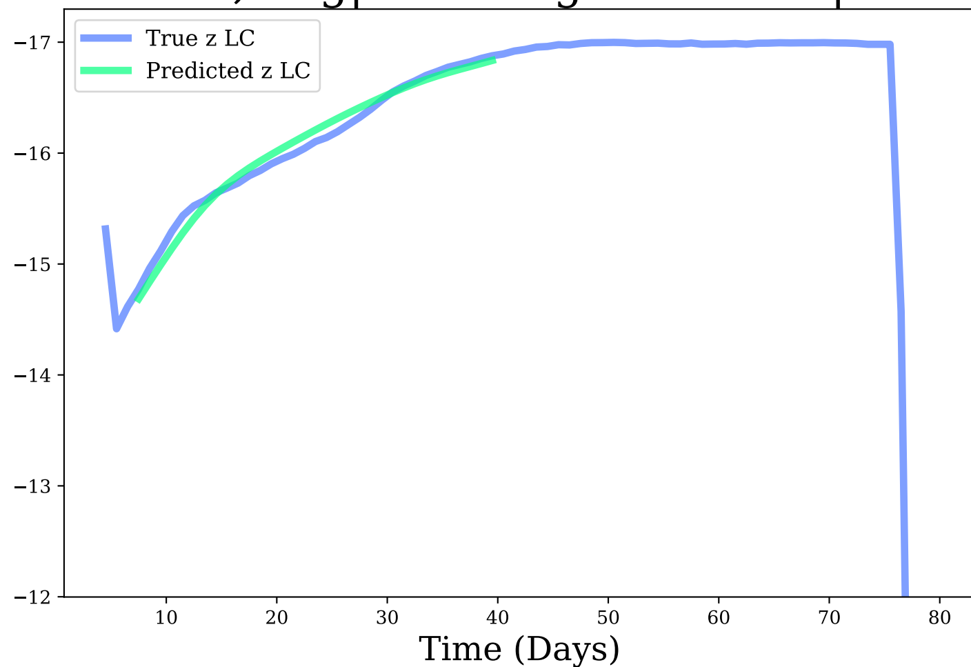
z-band, Avg|Max Mag Diff: 0.07 | 0.16
