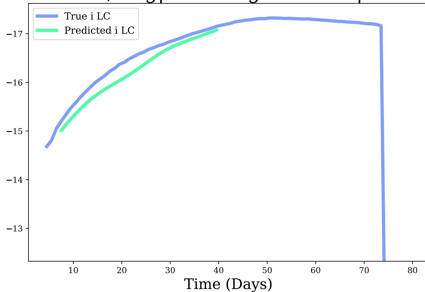
i-band, Avg|Max Mag Diff: 0.2 | 0.34
