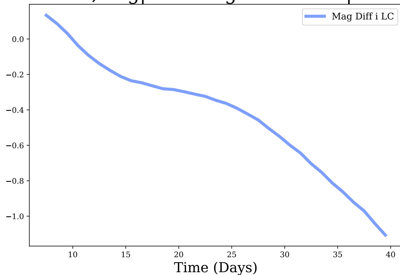
i-band, Avg|Max Mag Diff: -0.43 | 1.11
