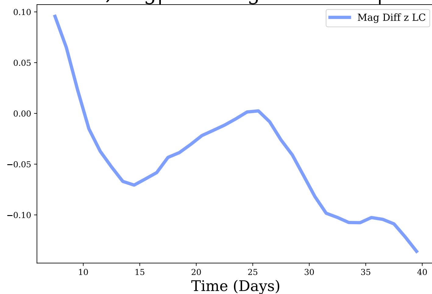
z-band, Avg|Max Mag Diff: -0.05 | 0.14
