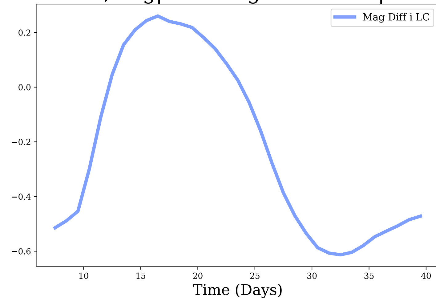
i-band, Avg|Max Mag Diff: -0.22 | 0.61
