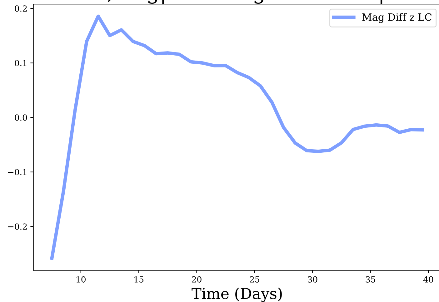
z-band, Avg|Max Mag Diff: 0.03 | 0.26
