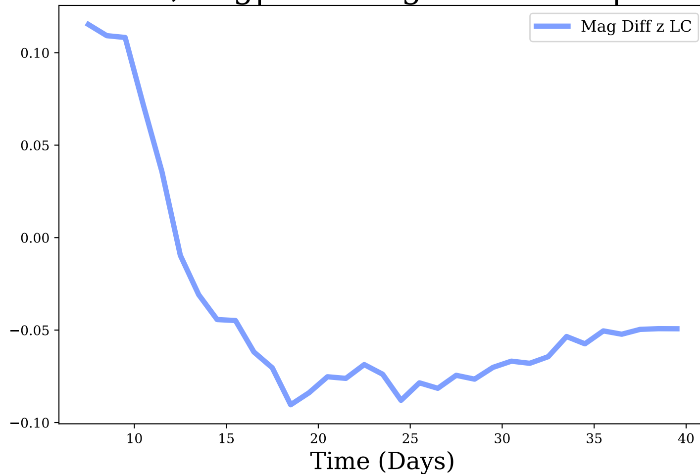
z-band, Avg|Max Mag Diff: -0.04 | 0.12
