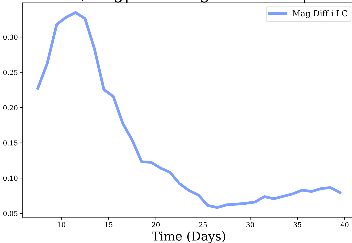
i-band, Avg|Max Mag Diff: 0.14 | 0.33
