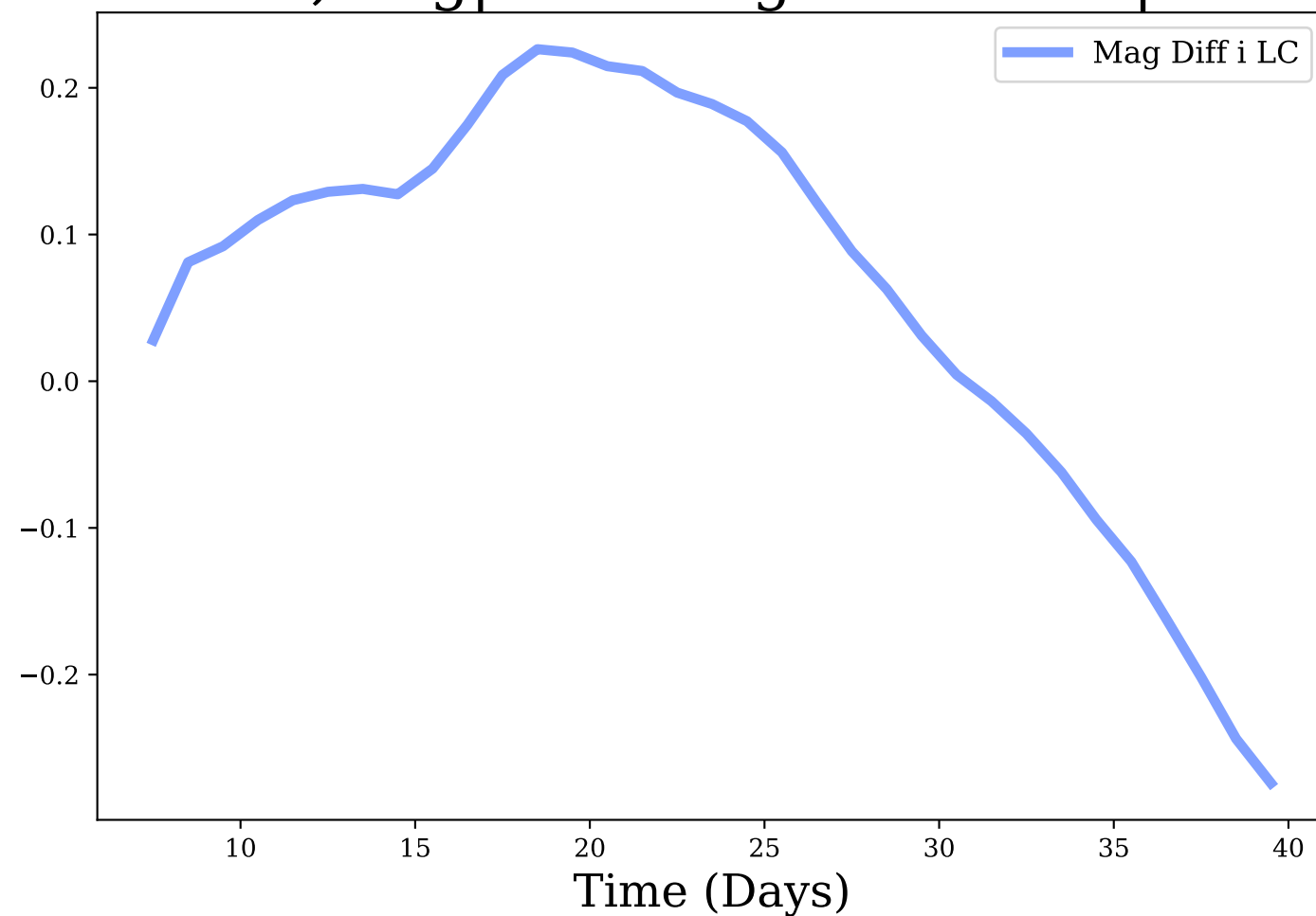
i-band, Avg|Max Mag Diff: 0.06 | 0.27
