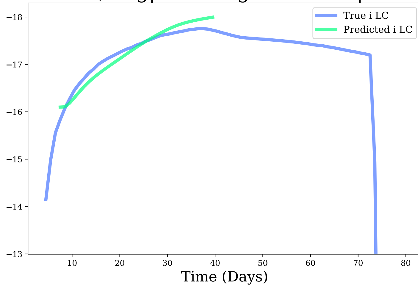
i-band, Avg|Max Mag Diff: 0.14 | 0.27
