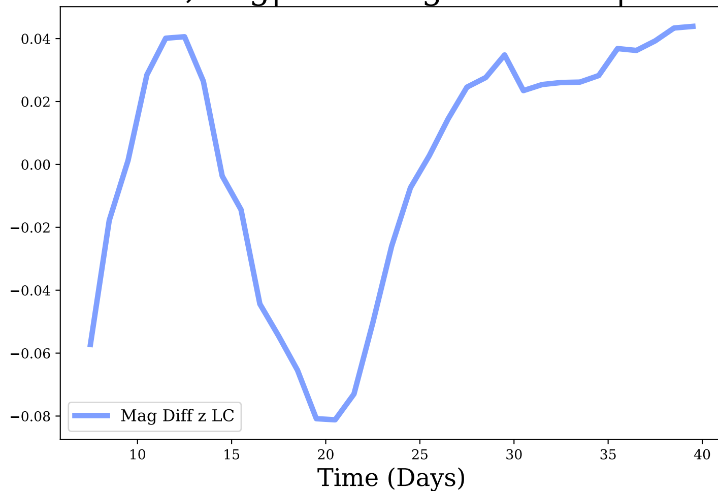
z-band, Avg|Max Mag Diff: -0.0 | 0.08
