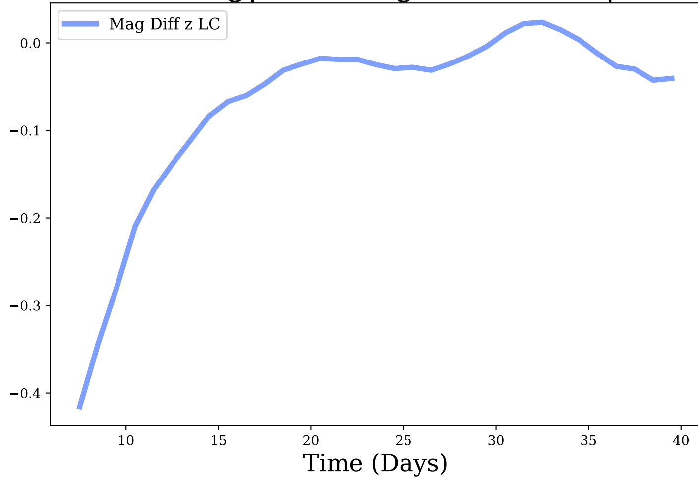
z-band, Avg|Max Mag Diff: -0.07 | 0.42
