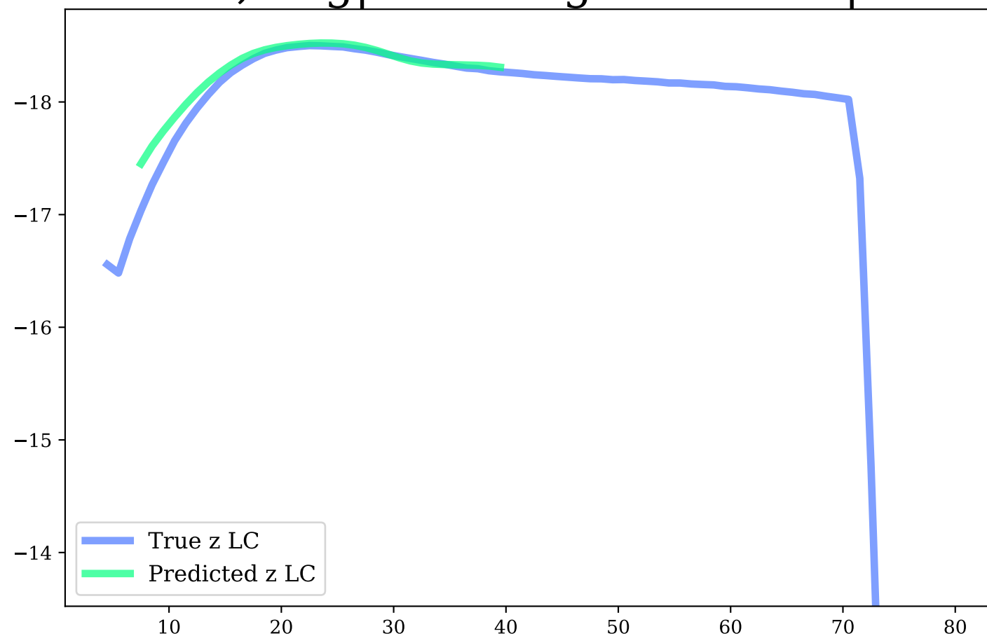
z-band, Avg|Max Mag Diff: 0.07 | 0.42
