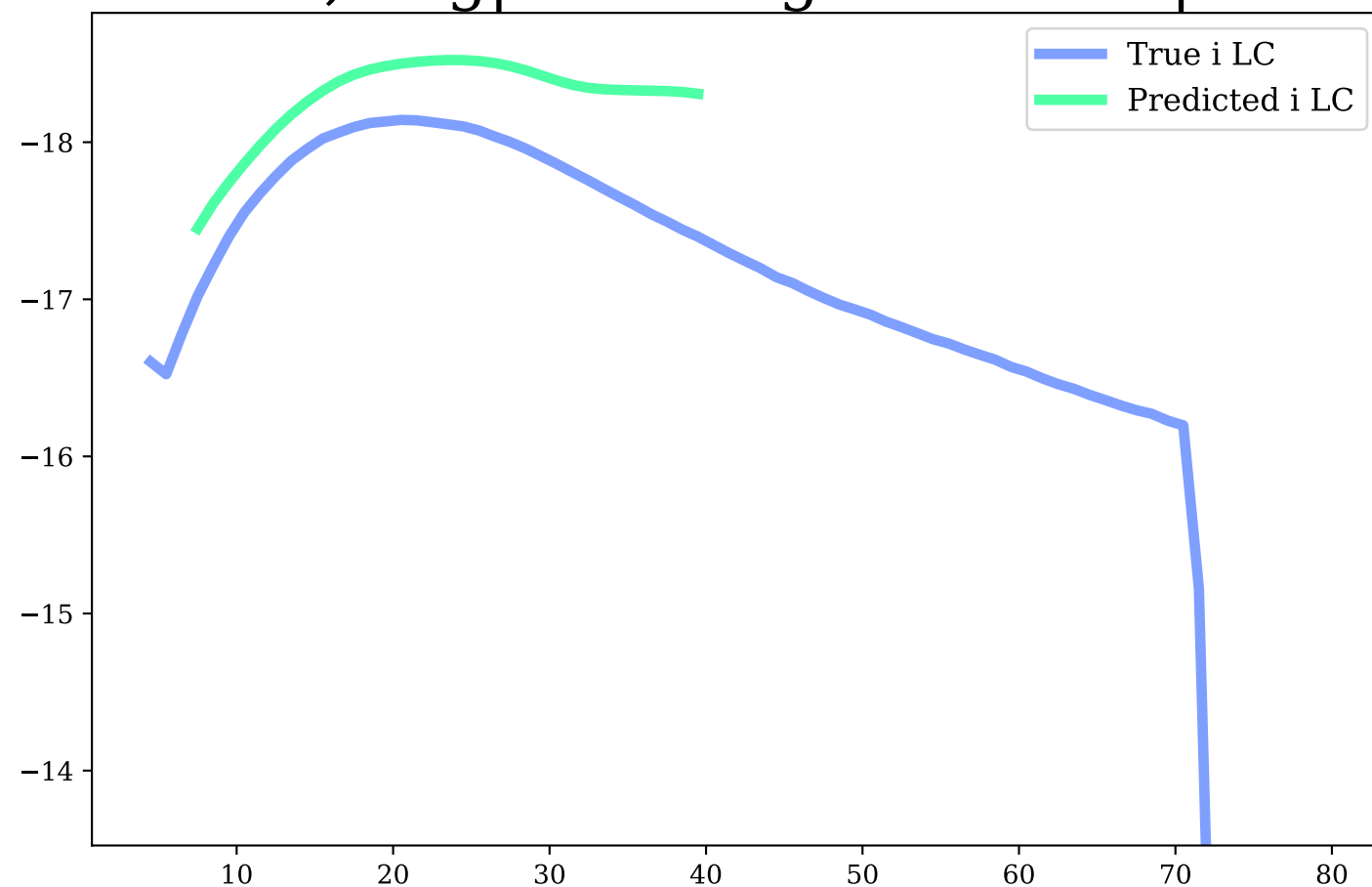
i-band, Avg|Max Mag Diff: 0.48 | 0.91
