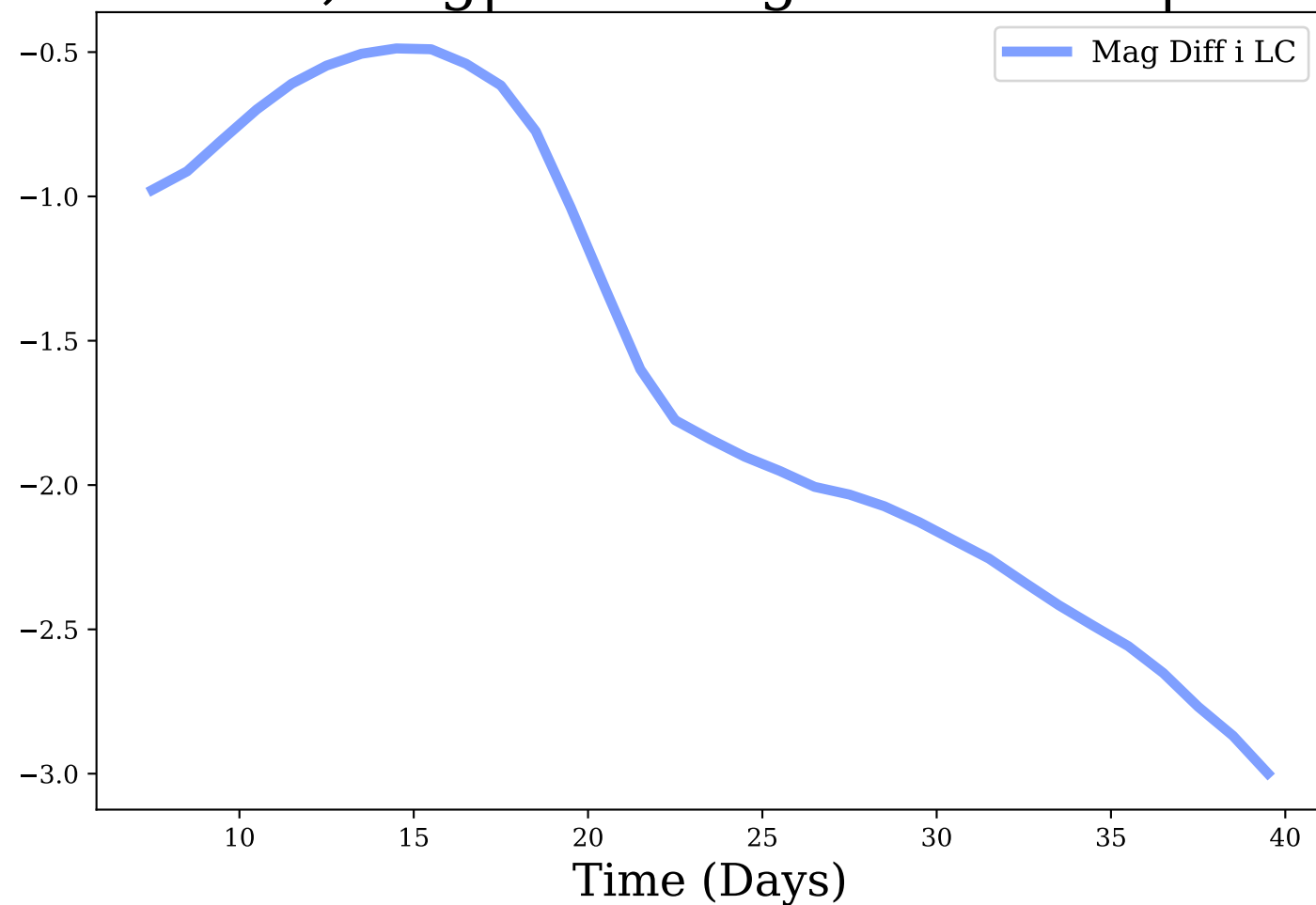
i-band, Avg|Max Mag Diff: -1.61 | 3.0
