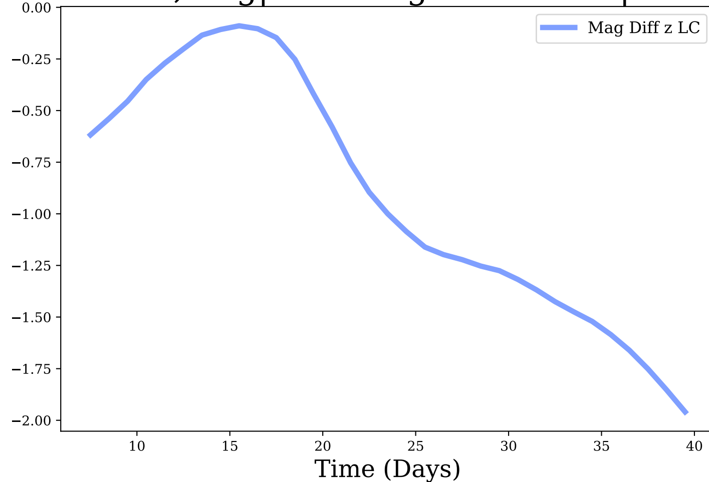
z-band, Avg|Max Mag Diff: -0.91 | 1.96
