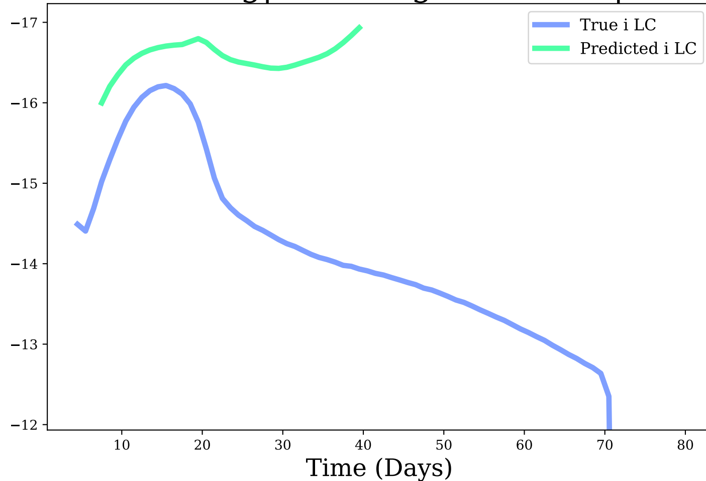
i-band, Avg|Max Mag Diff: 1.61 | 3.0
