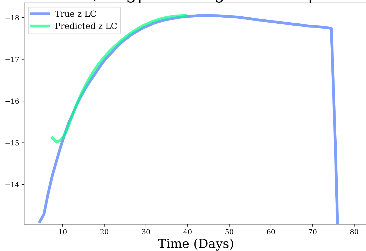
z-band, Avg|Max Mag Diff: 0.1 | 0.91
