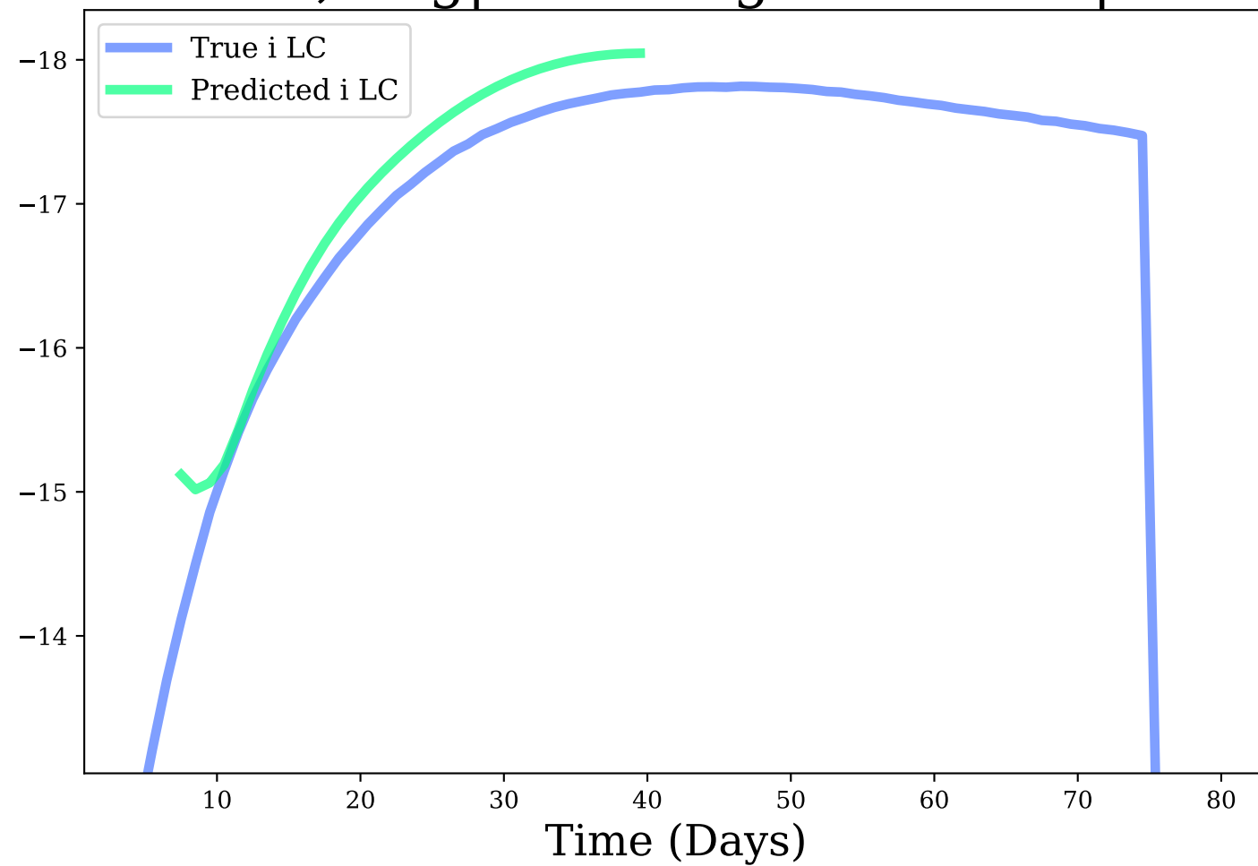
i-band, Avg|Max Mag Diff: 0.27 | 1.0
