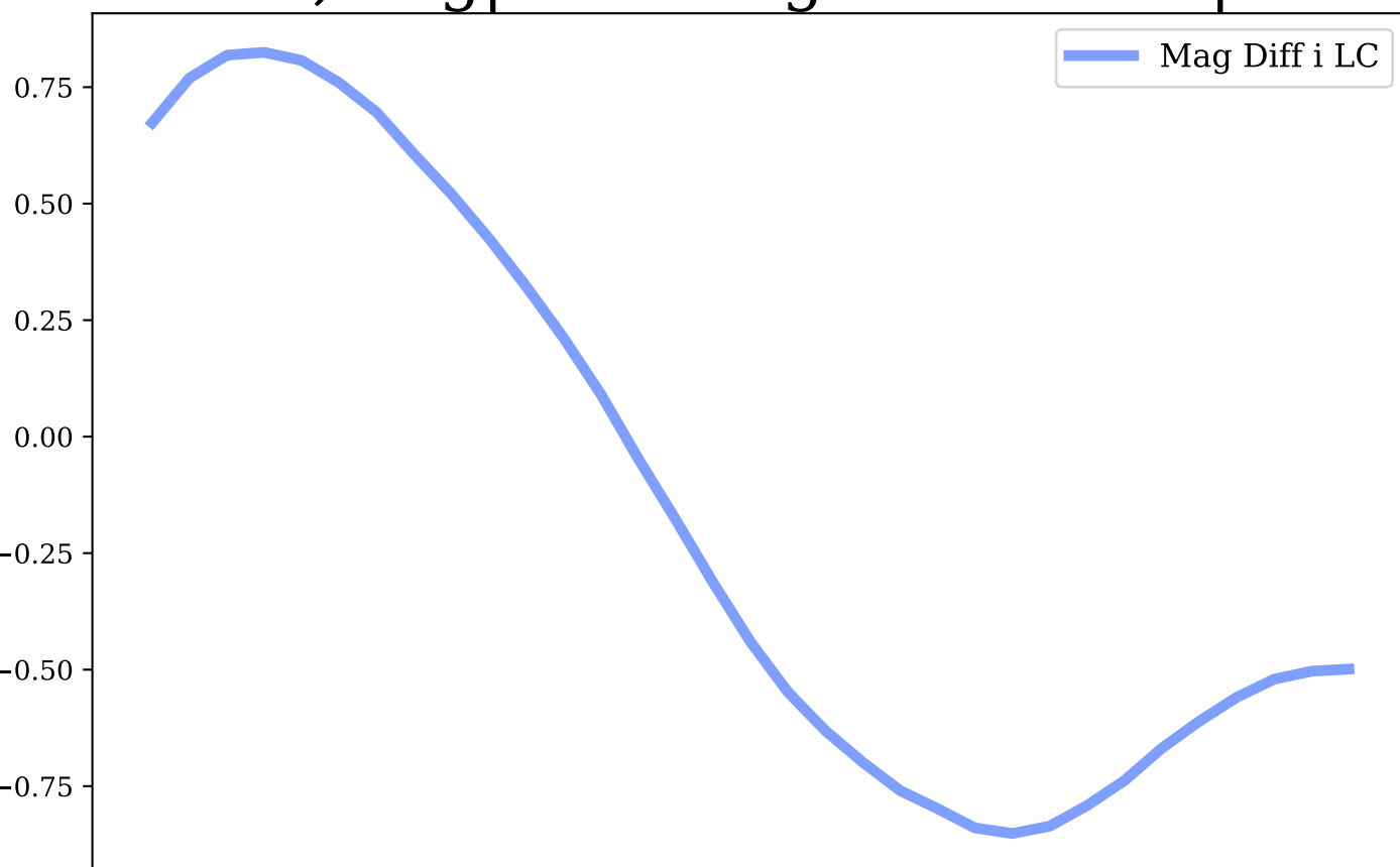
i-band, Avg|Max Mag Diff: -0.13 | 0.85
