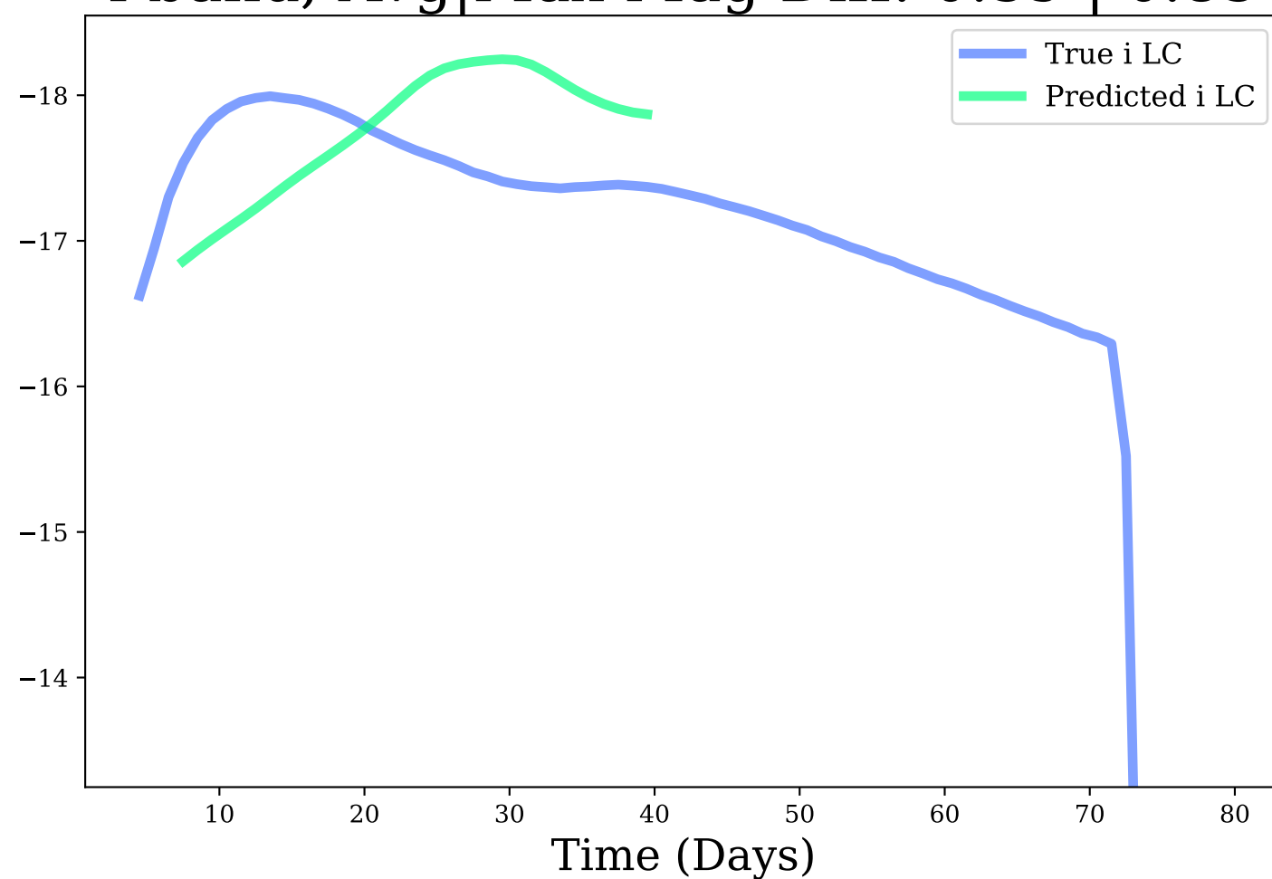
i-band, Avg|Max Mag Diff: 0.59 | 0.85
