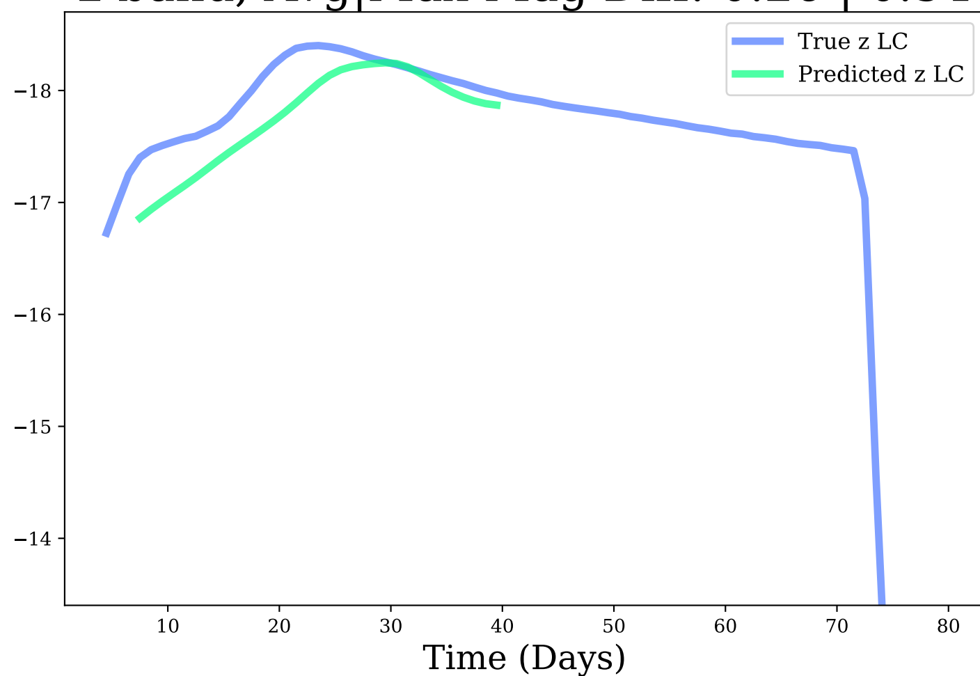
z-band, Avg|Max Mag Diff: 0.26 | 0.54
