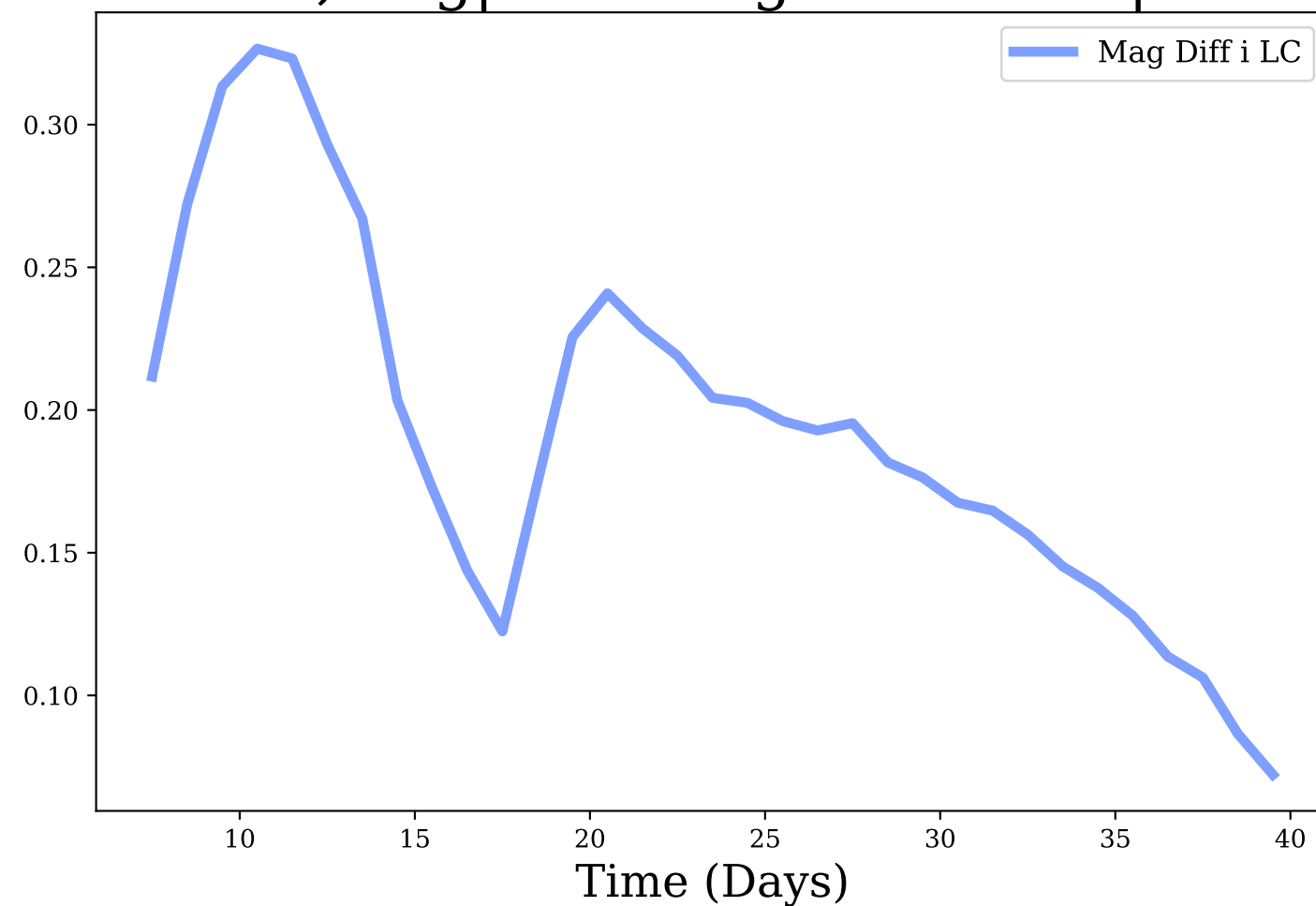
i-band, Avg|Max Mag Diff: 0.19 | 0.33
