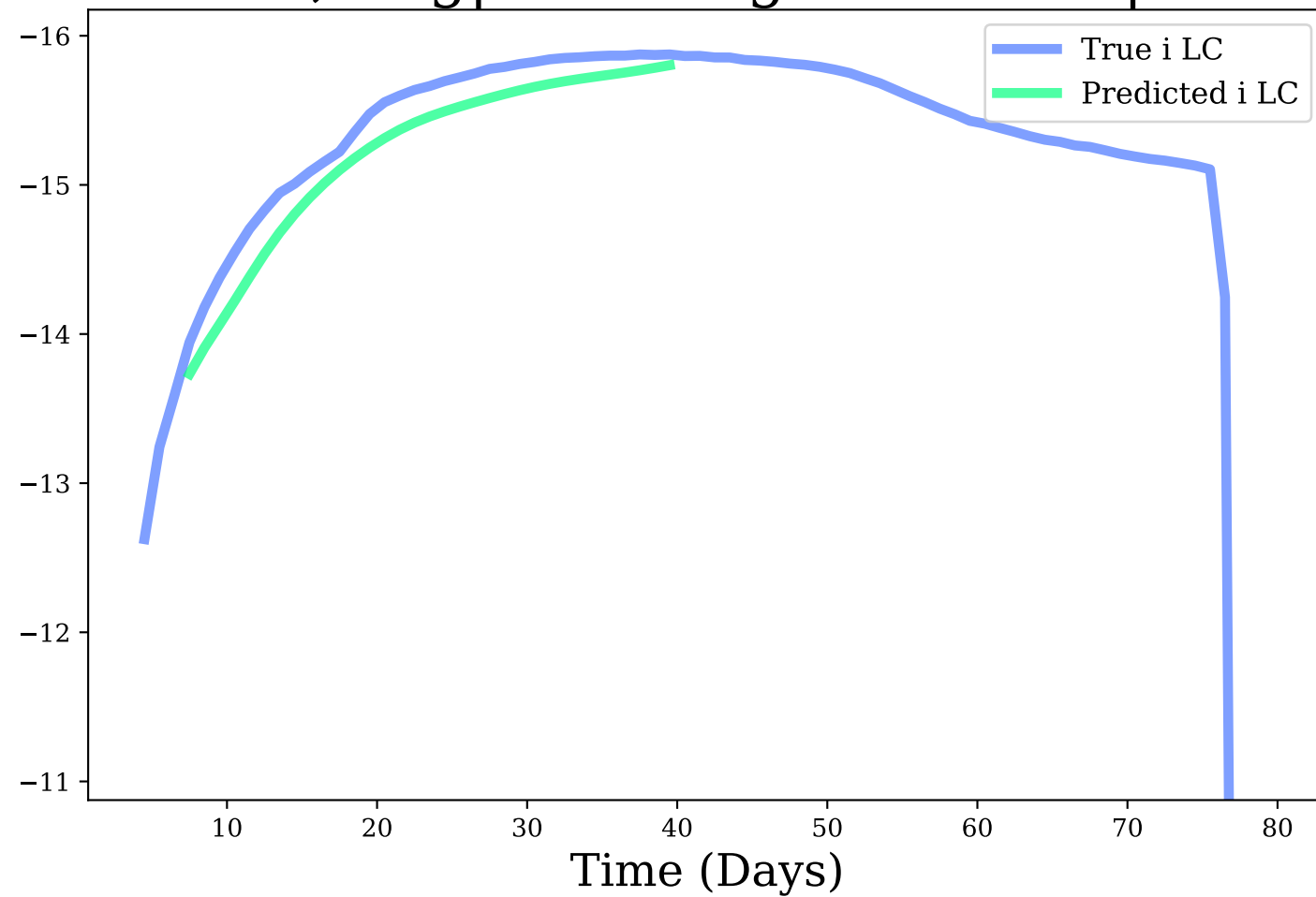
i-band, Avg|Max Mag Diff: 0.19 | 0.33
