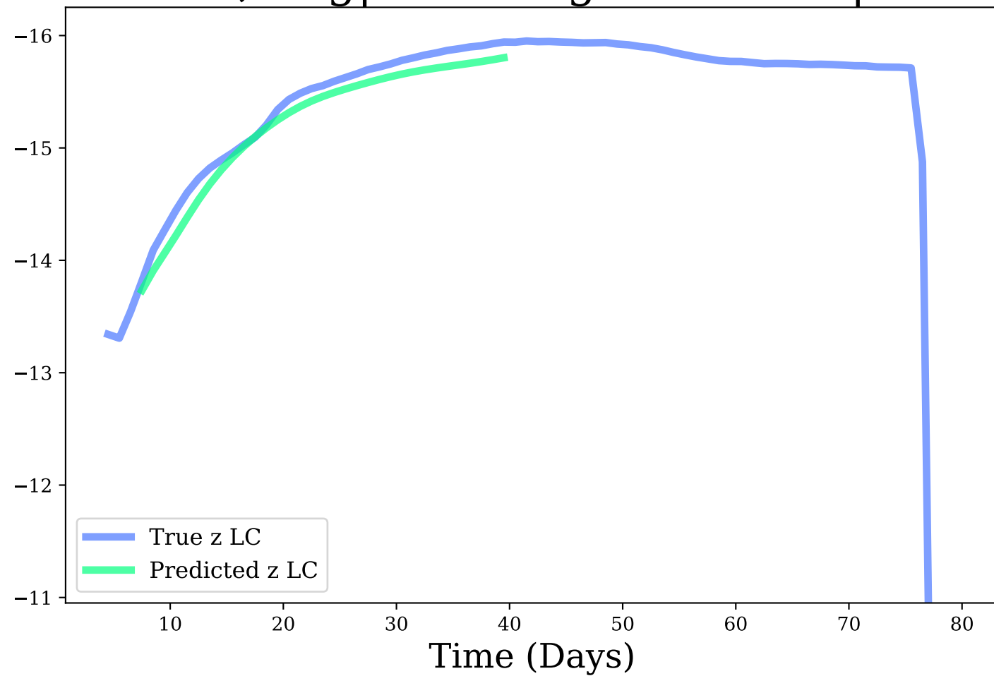
z-band, Avg|Max Mag Diff: 0.12 | 0.22
