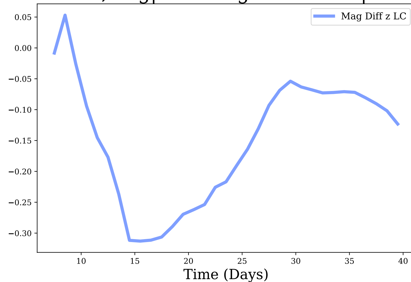
z-band, Avg|Max Mag Diff: -0.15 | 0.31
