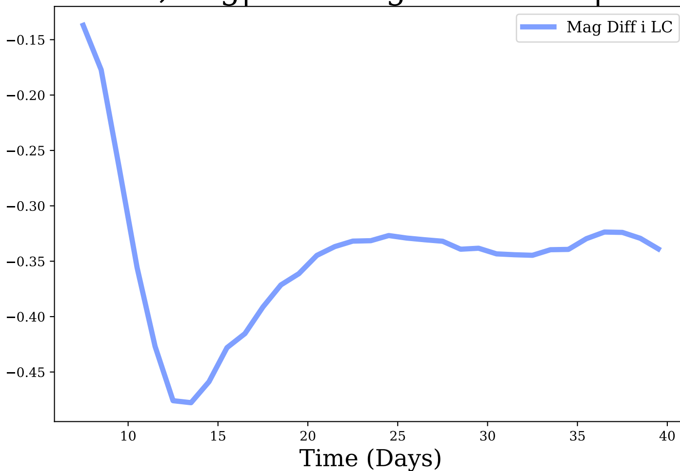
i-band, Avg|Max Mag Diff: -0.35 | 0.48
