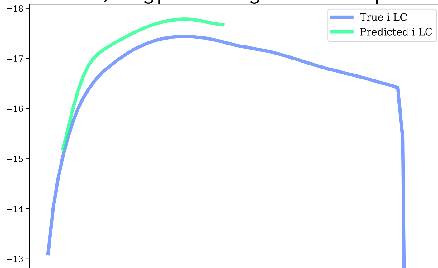
i-band, Avg|Max Mag Diff: 0.35 | 0.48
